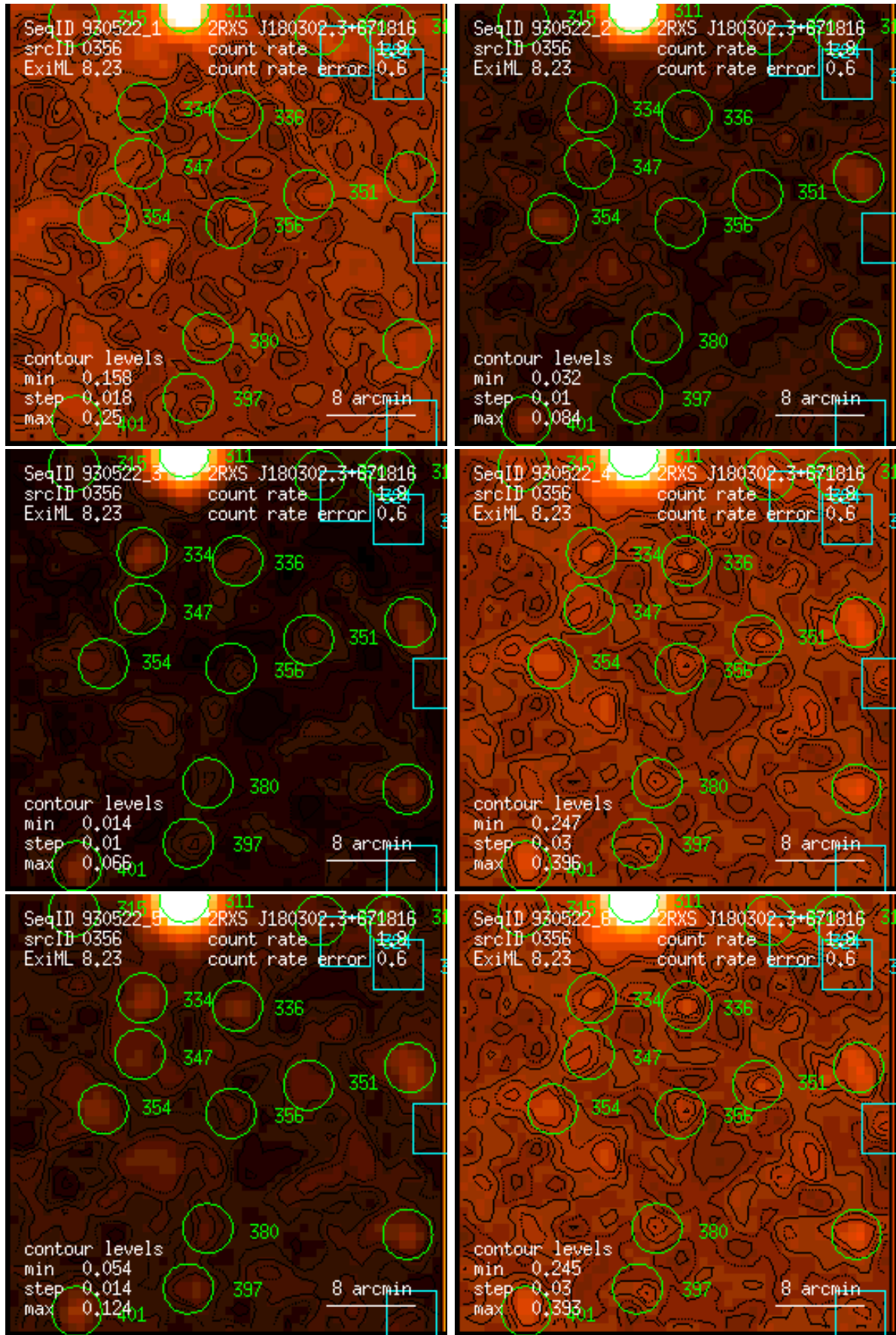
Figure 356: RASS 930522: detection 0356: band rate images, Gaussian filter: (1) PSPC channels 11 – 41, (2) 52 – 90, (3) 91 – 201, (4) 11 – 235, (5) 52 – 201, (6) 11 – 201. Broad band rates in counts/ks. Band rate contour levels in counts/ks/arcmin 2 .
