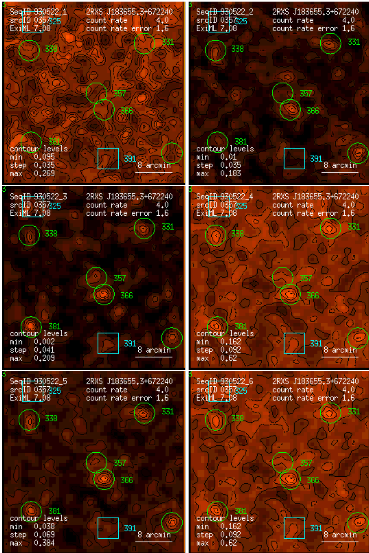
Figure 357: RASS 930522: detection 0357: band rate images, Gaussian filter: (1) PSPC channels 11 – 41, (2) 52 – 90, (3) 91 – 201, (4) 11 – 235, (5) 52 – 201, (6) 11 – 201. Broad band rates in counts/ks. Band rate contour levels in counts/ks/arcmin 2 .
