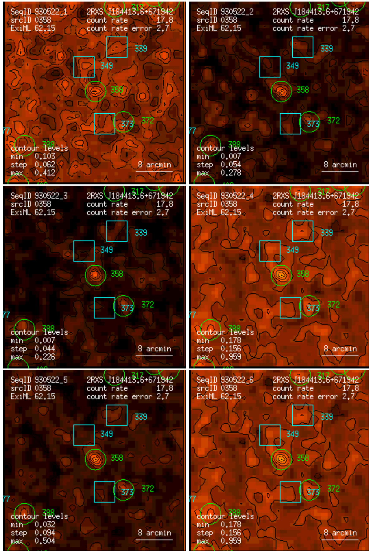
Figure 358: RASS 930522: detection 0358: band rate images, Gaussian filter: (1) PSPC channels 11 – 41, (2) 52 – 90, (3) 91 – 201, (4) 11 – 235, (5) 52 – 201, (6) 11 – 201. Broad band rates in counts/ks. Band rate contour levels in counts/ks/arcmin 2 .
