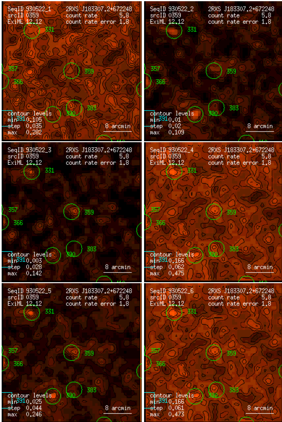
Figure 359: RASS 930522: detection 0359: band rate images, Gaussian filter: (1) PSPC channels 11 – 41, (2) 52 – 90, (3) 91 – 201, (4) 11 – 235, (5) 52 – 201, (6) 11 – 201. Broad band rates in counts/ks. Band rate contour levels in counts/ks/arcmin 2 .
