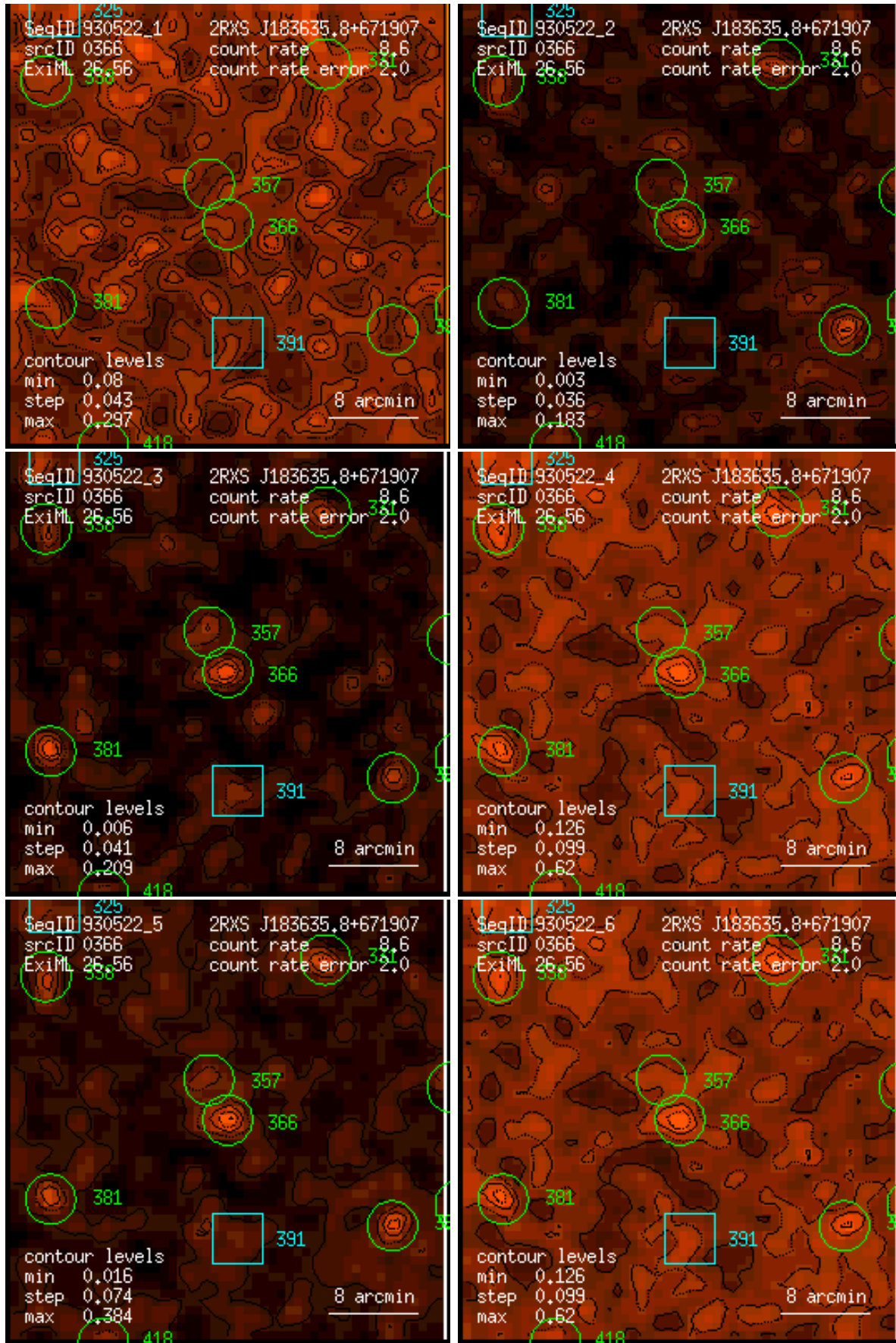
Figure 366: RASS 930522: detection 0366: band rate images, Gaussian filter: (1) PSPC channels 11 – 41, (2) 52 – 90, (3) 91 – 201, (4) 11 – 235, (5) 52 – 201, (6) 11 – 201. Broad band rates in counts/ks. Band rate contour levels in counts/ks/arcmin 2 .
