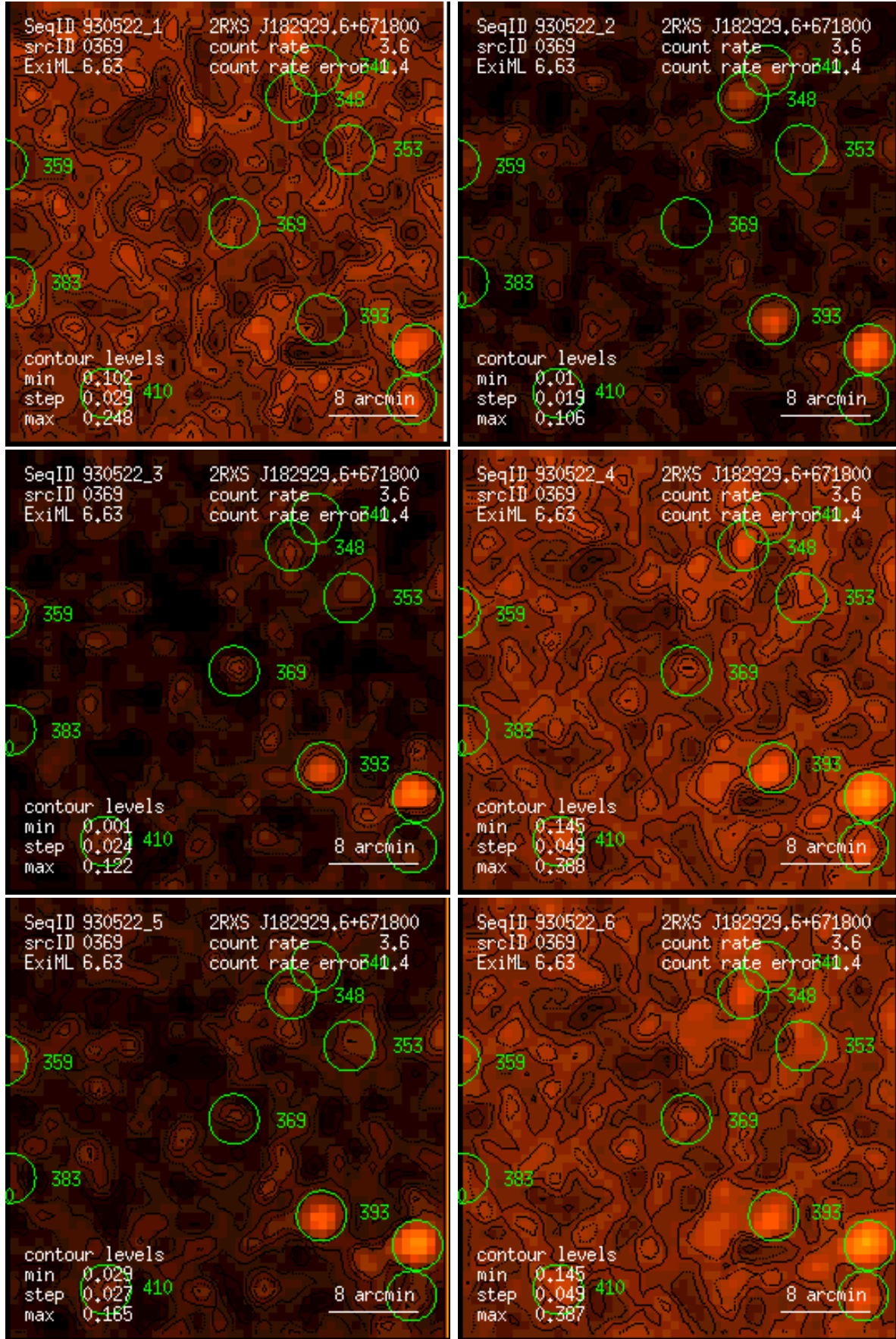
Figure 369: RASS 930522: detection 0369: band rate images, Gaussian filter: (1) PSPC channels 11 – 41, (2) 52 – 90, (3) 91 – 201, (4) 11 – 235, (5) 52 – 201, (6) 11 – 201. Broad band rates in counts/ks. Band rate contour levels in counts/ks/arcmin 2 .
