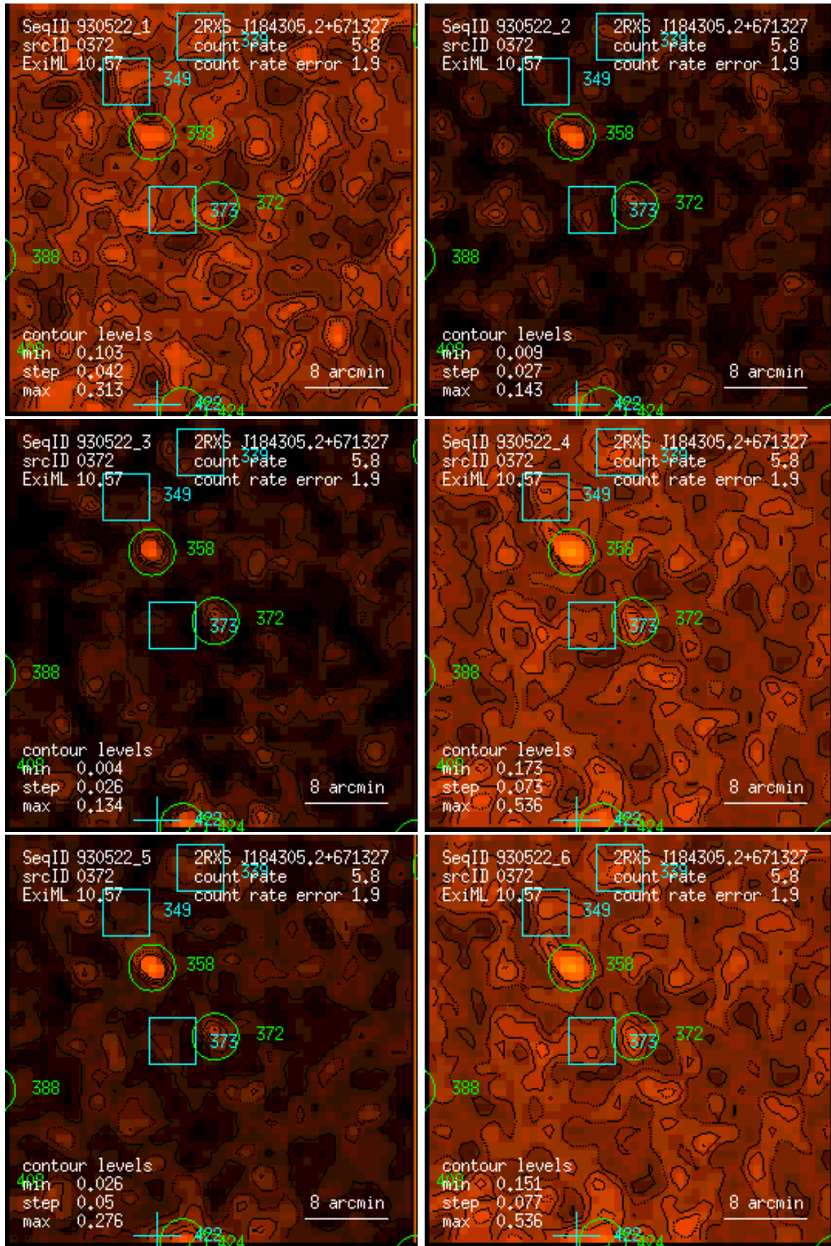
Figure 372: RASS 930522: detection 0372: band rate images, Gaussian filter: (1) PSPC channels 11 – 41, (2) 52 – 90, (3) 91 – 201, (4) 11 – 235, (5) 52 – 201, (6) 11 – 201. Broad band rates in counts/ks. Band rate contour levels in counts/ks/arcmin 2 .
