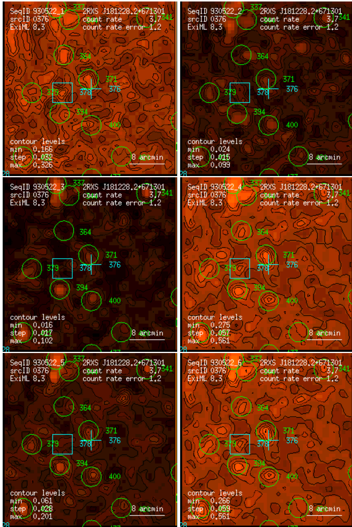
Figure 376: RASS 930522: detection 0376: band rate images, Gaussian filter: (1) PSPC channels 11 – 41, (2) 52 – 90, (3) 91 – 201, (4) 11 – 235, (5) 52 – 201, (6) 11 – 201. Broad band rates in counts/ks. Band rate contour levels in counts/ks/arcmin 2 .
