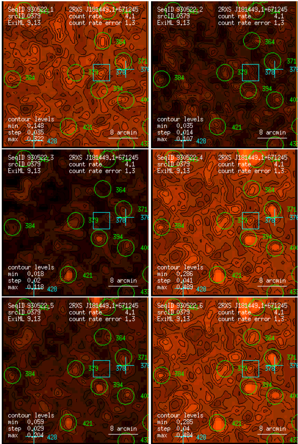
Figure 379: RASS 930522: detection 0379: band rate images, Gaussian filter: (1) PSPC channels 11 – 41, (2) 52 – 90, (3) 91 – 201, (4) 11 – 235, (5) 52 – 201, (6) 11 – 201. Broad band rates in counts/ks. Band rate contour levels in counts/ks/arcmin 2 .
