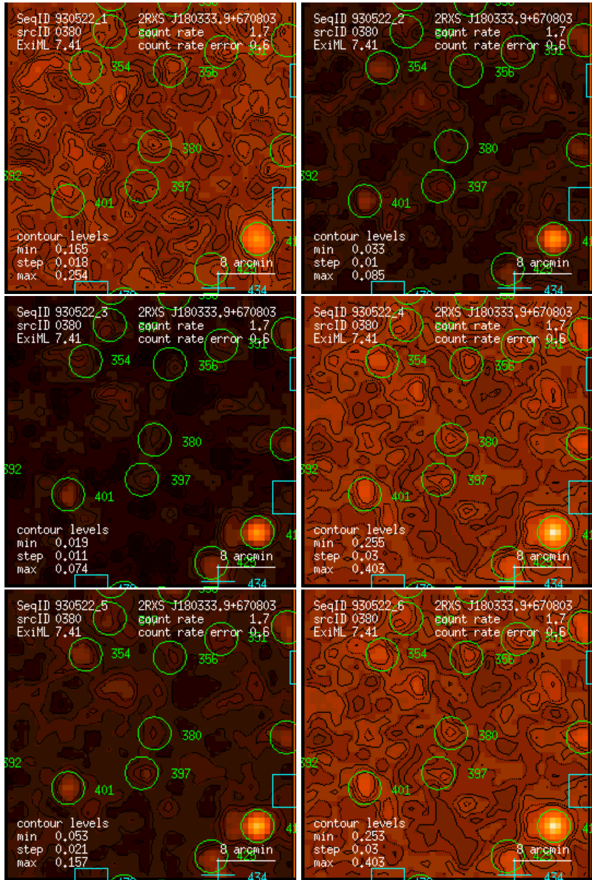
Figure 380: RASS 930522: detection 0380: band rate images, Gaussian filter: (1) PSPC channels 11 – 41, (2) 52 – 90, (3) 91 – 201, (4) 11 – 235, (5) 52 – 201, (6) 11 – 201. Broad band rates in counts/ks. Band rate contour levels in counts/ks/arcmin 2 .
