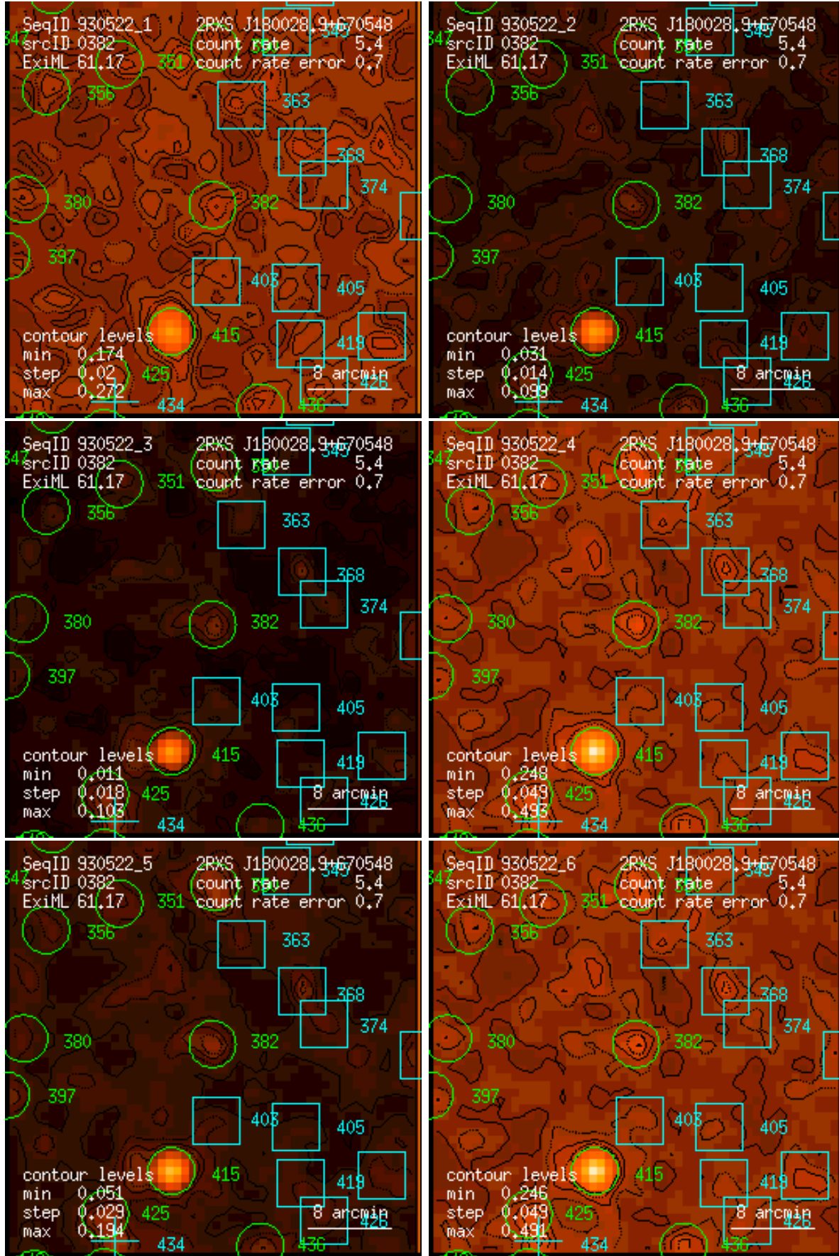
Figure 382: RASS 930522: detection 0382: band rate images, Gaussian filter: (1) PSPC channels 11 – 41, (2) 52 – 90, (3) 91 – 201, (4) 11 – 235, (5) 52 – 201, (6) 11 – 201. Broad band rates in counts/ks. Band rate contour levels in counts/ks/arcmin 2 .
