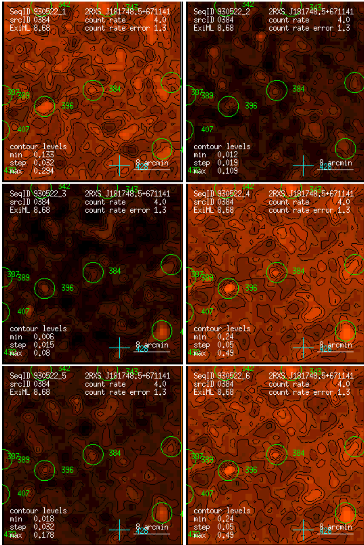
Figure 384: RASS 930522: detection 0384: band rate images, Gaussian filter: (1) PSPC channels 11 – 41, (2) 52 – 90, (3) 91 – 201, (4) 11 – 235, (5) 52 – 201, (6) 11 – 201. Broad band rates in counts/ks. Band rate contour levels in counts/ks/arcmin 2 .
