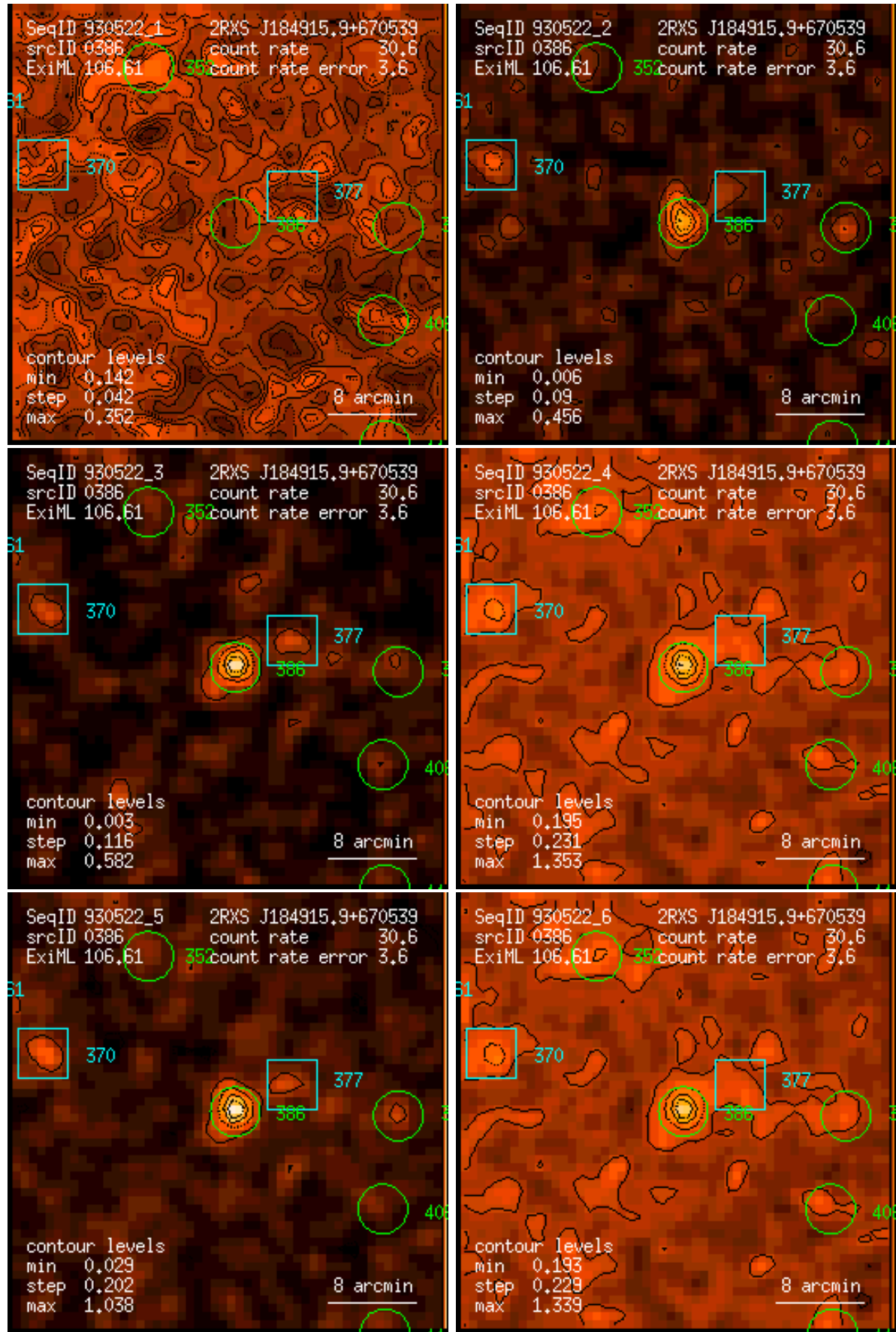
Figure 386: RASS 930522: detection 0386: band rate images, Gaussian filter: (1) PSPC channels 11 – 41, (2) 52 – 90, (3) 91 – 201, (4) 11 – 235, (5) 52 – 201, (6) 11 – 201. Broad band rates in counts/ks. Band rate contour levels in counts/ks/arcmin 2 .
