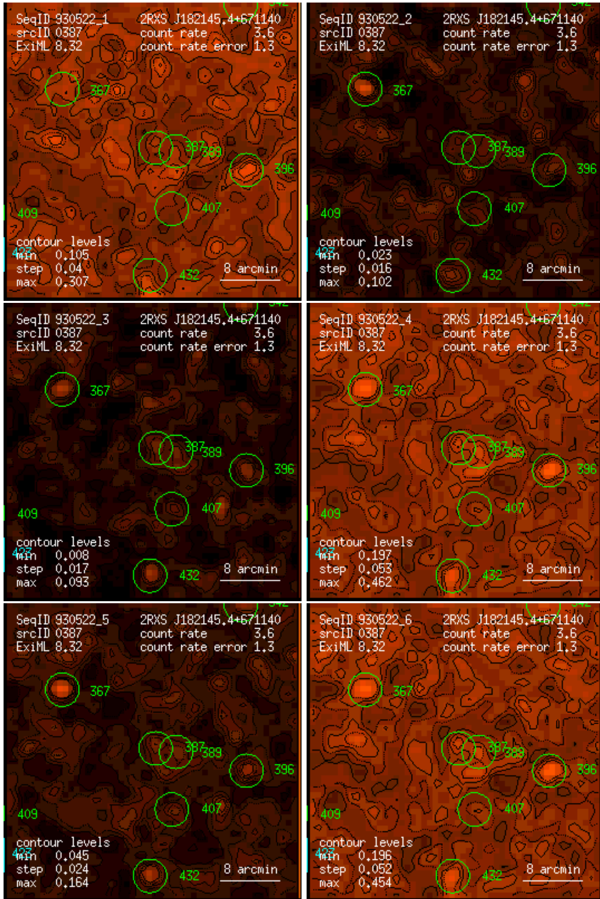
Figure 387: RASS 930522: detection 0387: band rate images, Gaussian filter: (1) PSPC channels 11 – 41, (2) 52 – 90, (3) 91 – 201, (4) 11 – 235, (5) 52 – 201, (6) 11 – 201. Broad band rates in counts/ks. Band rate contour levels in counts/ks/arcmin 2 .
