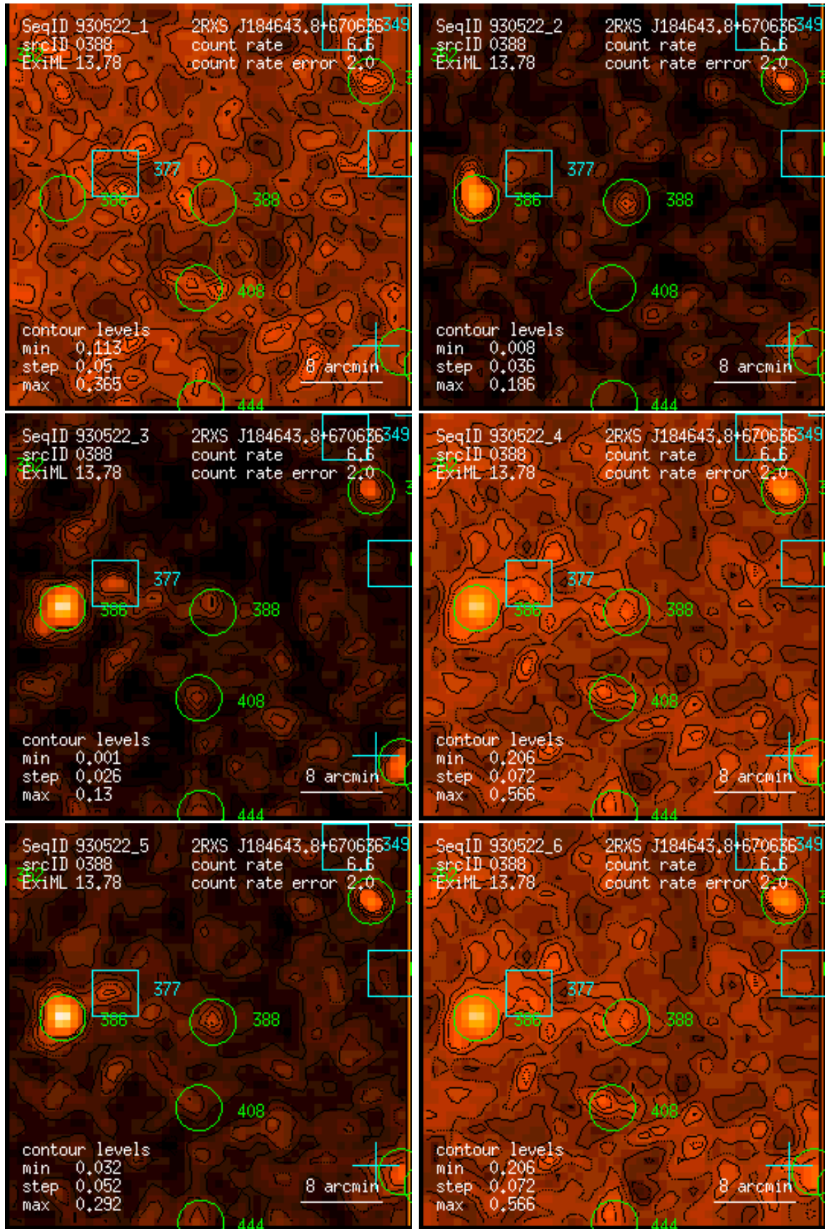
Figure 388: RASS 930522: detection 0388: band rate images, Gaussian filter: (1) PSPC channels 11 – 41, (2) 52 – 90, (3) 91 – 201, (4) 11 – 235, (5) 52 – 201, (6) 11 – 201. Broad band rates in counts/ks. Band rate contour levels in counts/ks/arcmin 2 .
