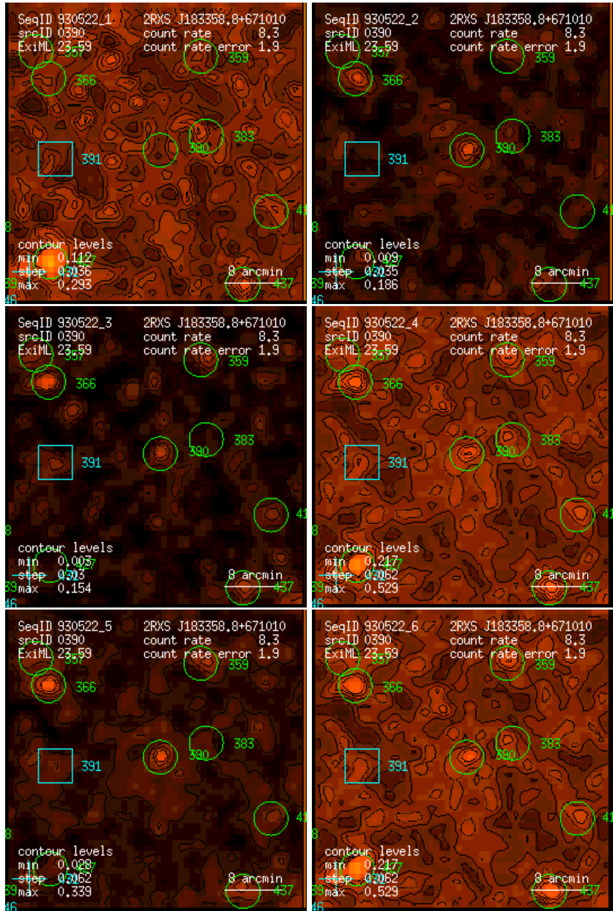
Figure 390: RASS 930522: detection 0390: band rate images, Gaussian filter: (1) PSPC channels 11 – 41, (2) 52 – 90, (3) 91 – 201, (4) 11 – 235, (5) 52 – 201, (6) 11 – 201. Broad band rates in counts/ks. Band rate contour levels in counts/ks/arcmin 2 .
