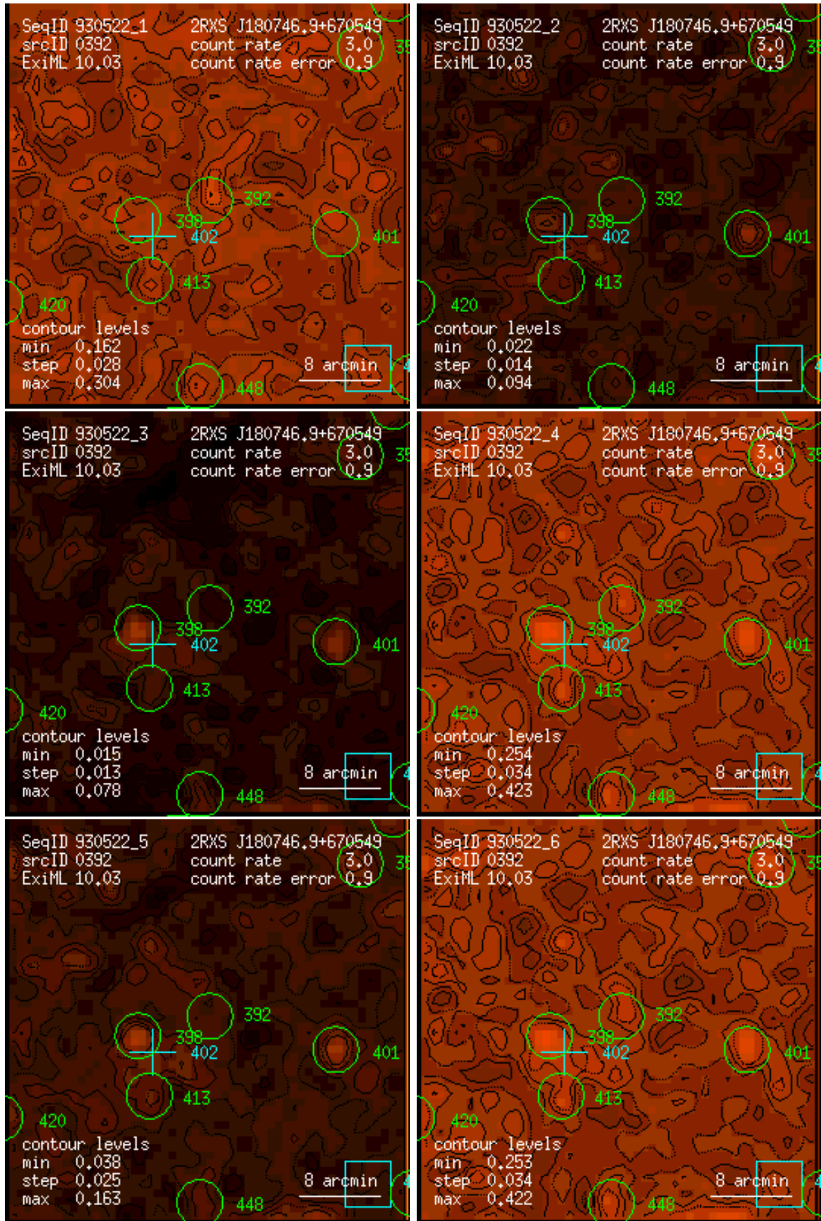
Figure 392: RASS 930522: detection 0392: band rate images, Gaussian filter: (1) PSPC channels 11 – 41, (2) 52 – 90, (3) 91 – 201, (4) 11 – 235, (5) 52 – 201, (6) 11 – 201. Broad band rates in counts/ks. Band rate contour levels in counts/ks/arcmin 2 .
