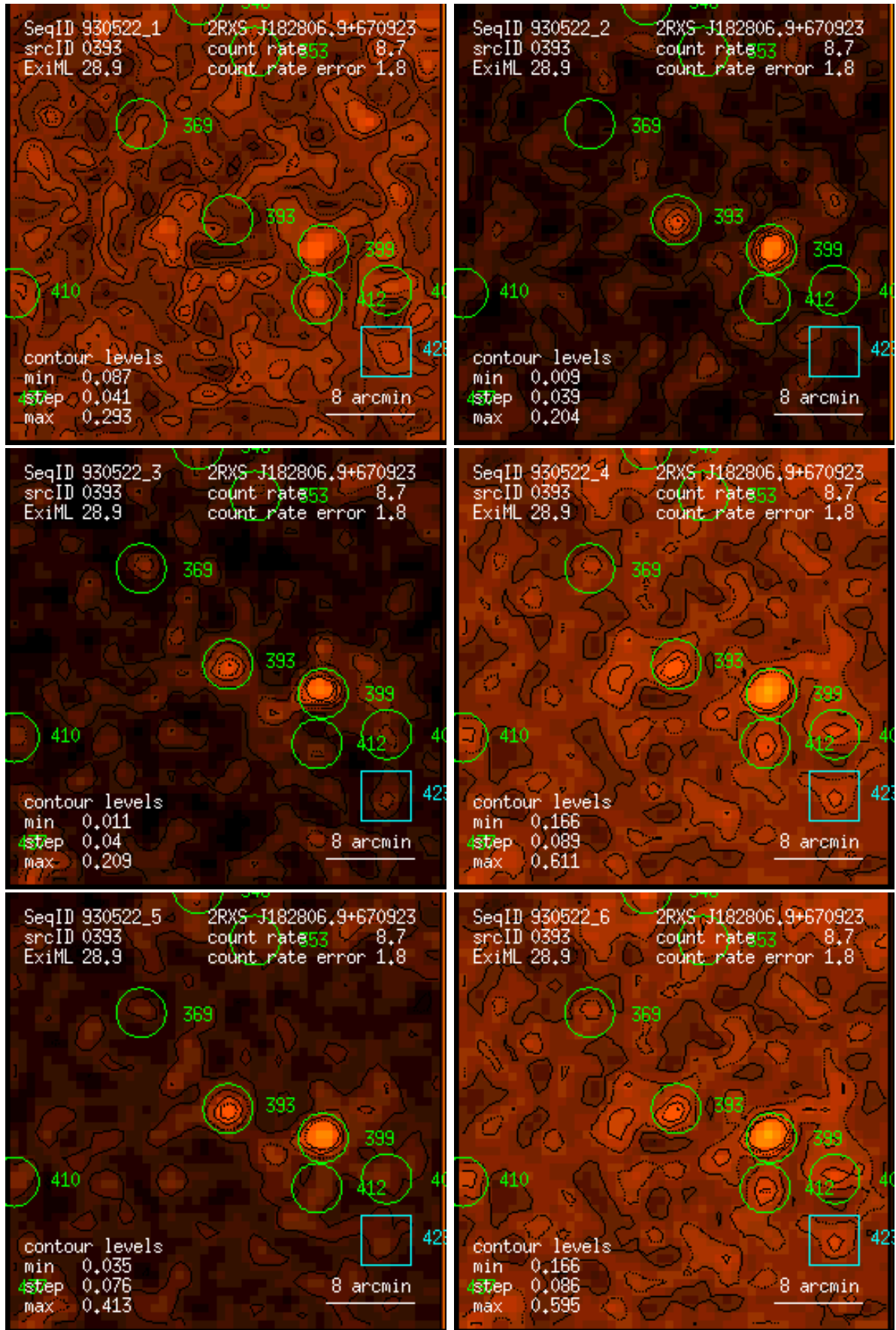
Figure 393: RASS 930522: detection 0393: band rate images, Gaussian filter: (1) PSPPC channels 11 – 41, (2) 52 – 90, (3) 91 – 201, (4) 11 – 235, (5) 52 – 201, (6) 11 – 201. Broad band rates in counts/ks. Band rate contour levels in counts/ks/arcmin 2 .
