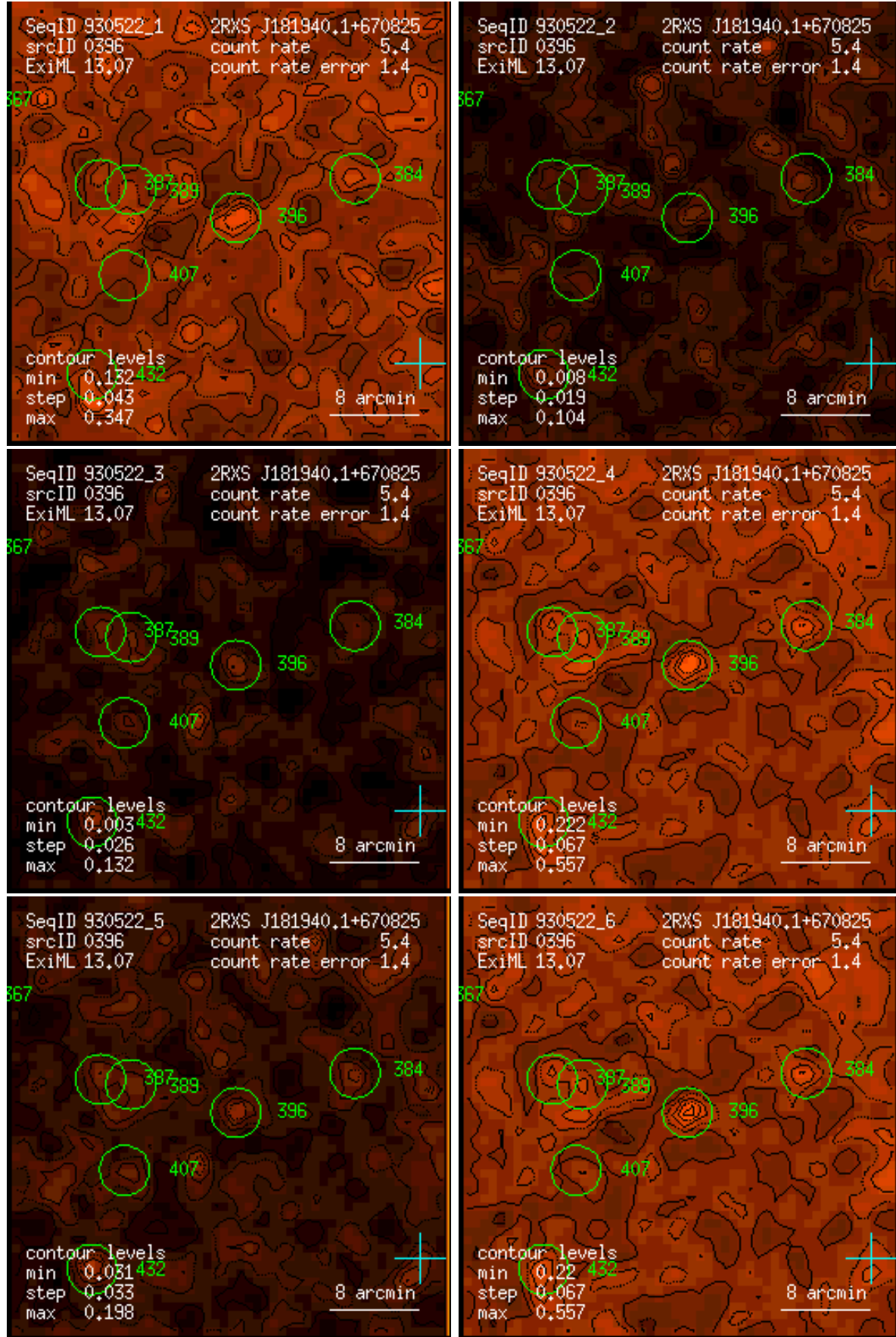
Figure 396: RASS 930522: detection 0396: band rate images, Gaussian filter: (1) PSPC channels 11 – 41, (2) 52 – 90, (3) 91 – 201, (4) 11 – 235, (5) 52 – 201, (6) 11 – 201. Broad band rates in counts/ks. Band rate contour levels in counts/ks/arcmin 2 .
