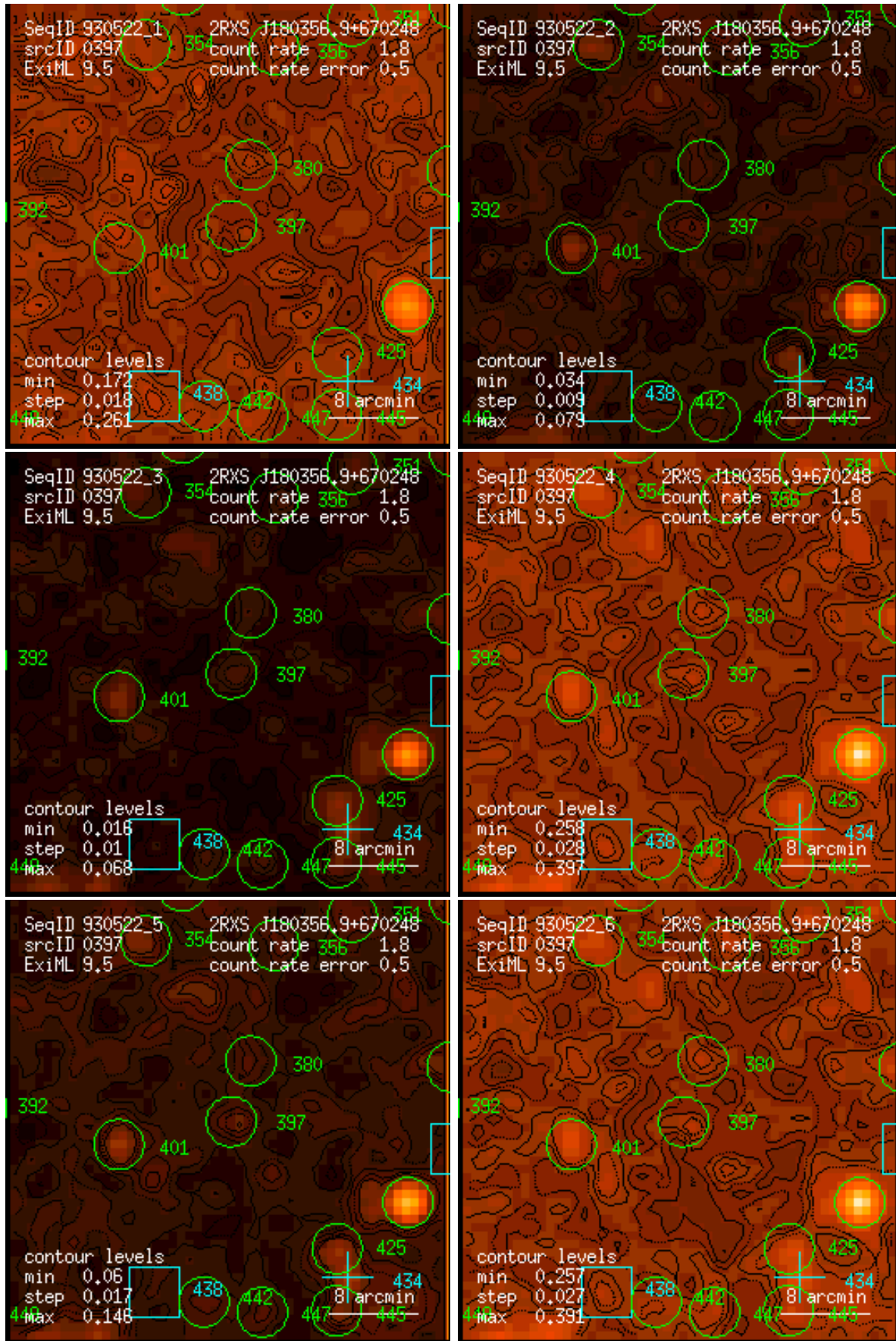
Figure 397: RASS 930522: detection 0397: band rate images, Gaussian filter: (1) PSPC channels 11 – 41, (2) 52 – 90, (3) 91 – 201, (4) 11 – 235, (5) 52 – 201, (6) 11 – 201. Broad band rates in counts/ks. Band rate contour levels in counts/ks/arcmin 2 .
