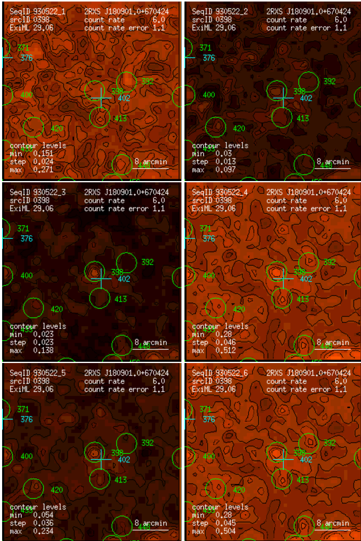
Figure 398: RASS 930522: detection 0398: band rate images, Gaussian filter: (1) PSPC channels 11 – 41, (2) 52 – 90, (3) 91 – 201, (4) 11 – 235, (5) 52 – 201, (6) 11 – 201. Broad band rates in counts/ks. Band rate contour levels in counts/ks/arcmin 2 .
