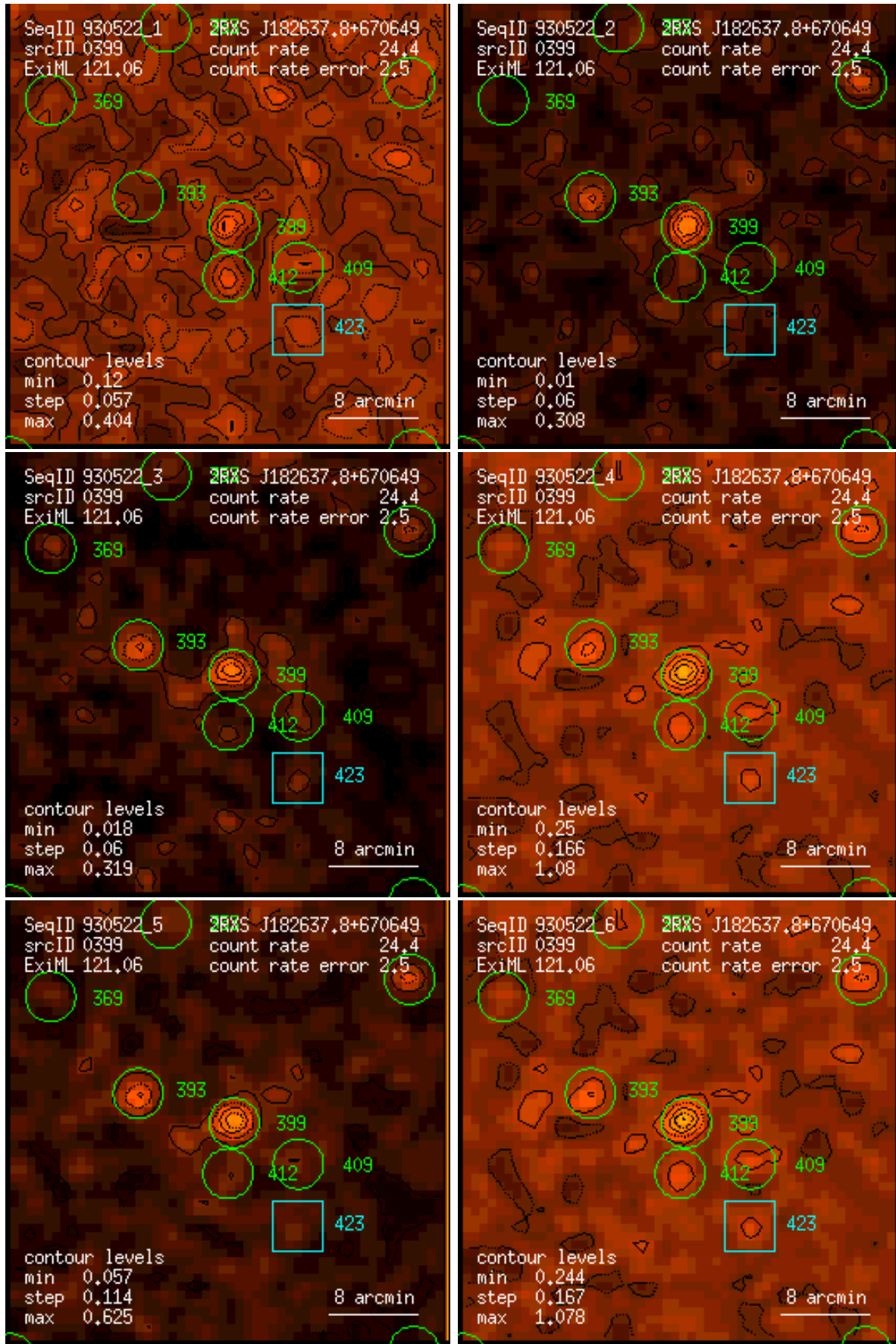
Figure 399: RASS 930522: detection 0399: band rate images, Gaussian filter: (1) PSPC channels 11 – 41, (2) 52 – 90, (3) 91 – 201, (4) 11 – 235, (5) 52 – 201, (6) 11 – 201. Broad band rates in counts/ks. Band rate contour levels in counts/ks/arcmin 2 .
