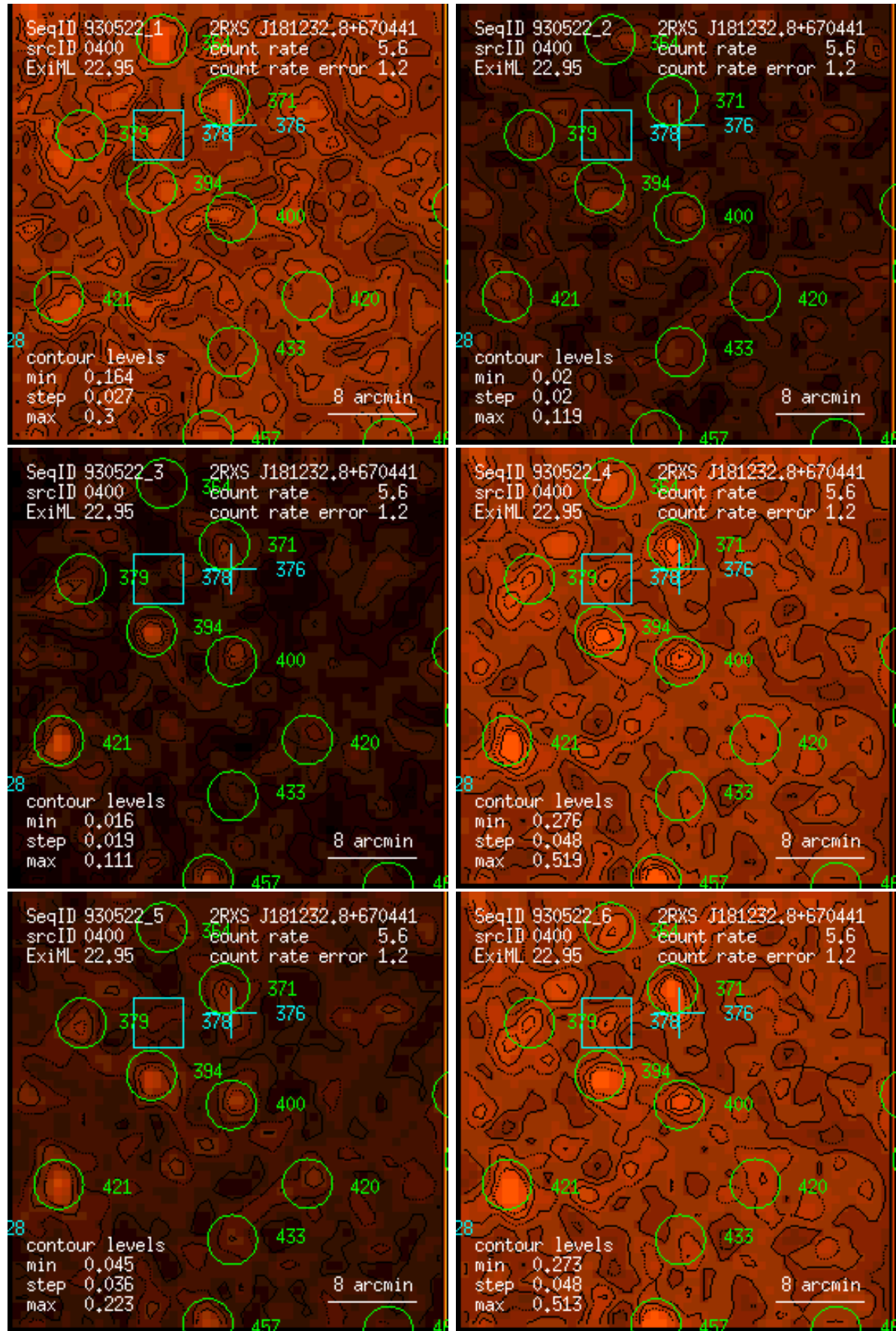
Figure 400: RASS 930522: detection 0400: band rate images, Gaussian filter: (1) PSPC channels 11 – 41, (2) 52 – 90, (3) 91 – 201, (4) 11 – 235, (5) 52 – 201, (6) 11 – 201. Broad band rates in counts/ks. Band rate contour levels in counts/ks/arcmin 2 .
