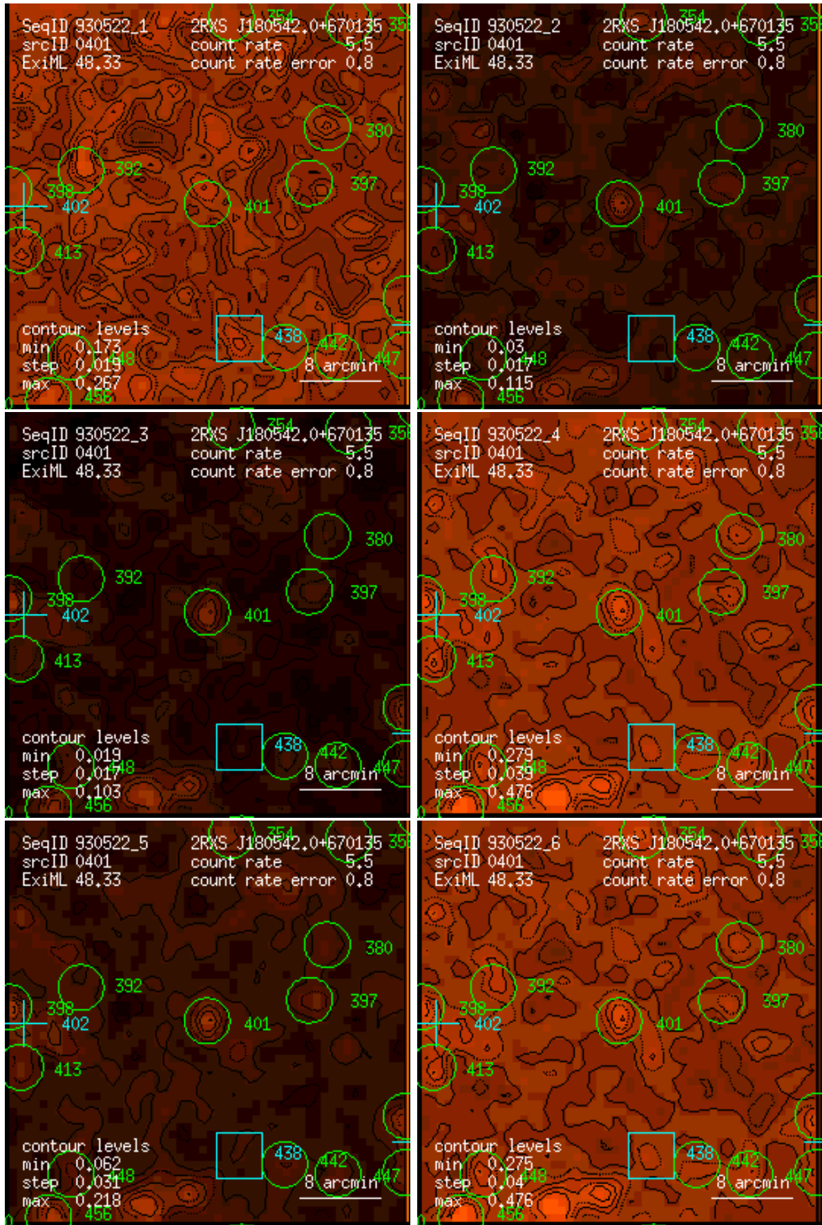
Figure 401: RASS 930522: detection 0401: band rate images, Gaussian filter: (1) PSPC channels 11 – 41, (2) 52 – 90, (3) 91 – 201, (4) 11 – 235, (5) 52 – 201, (6) 11 – 201. Broad band rates in counts/ks. Band rate contour levels in counts/ks/arcmin 2 .
