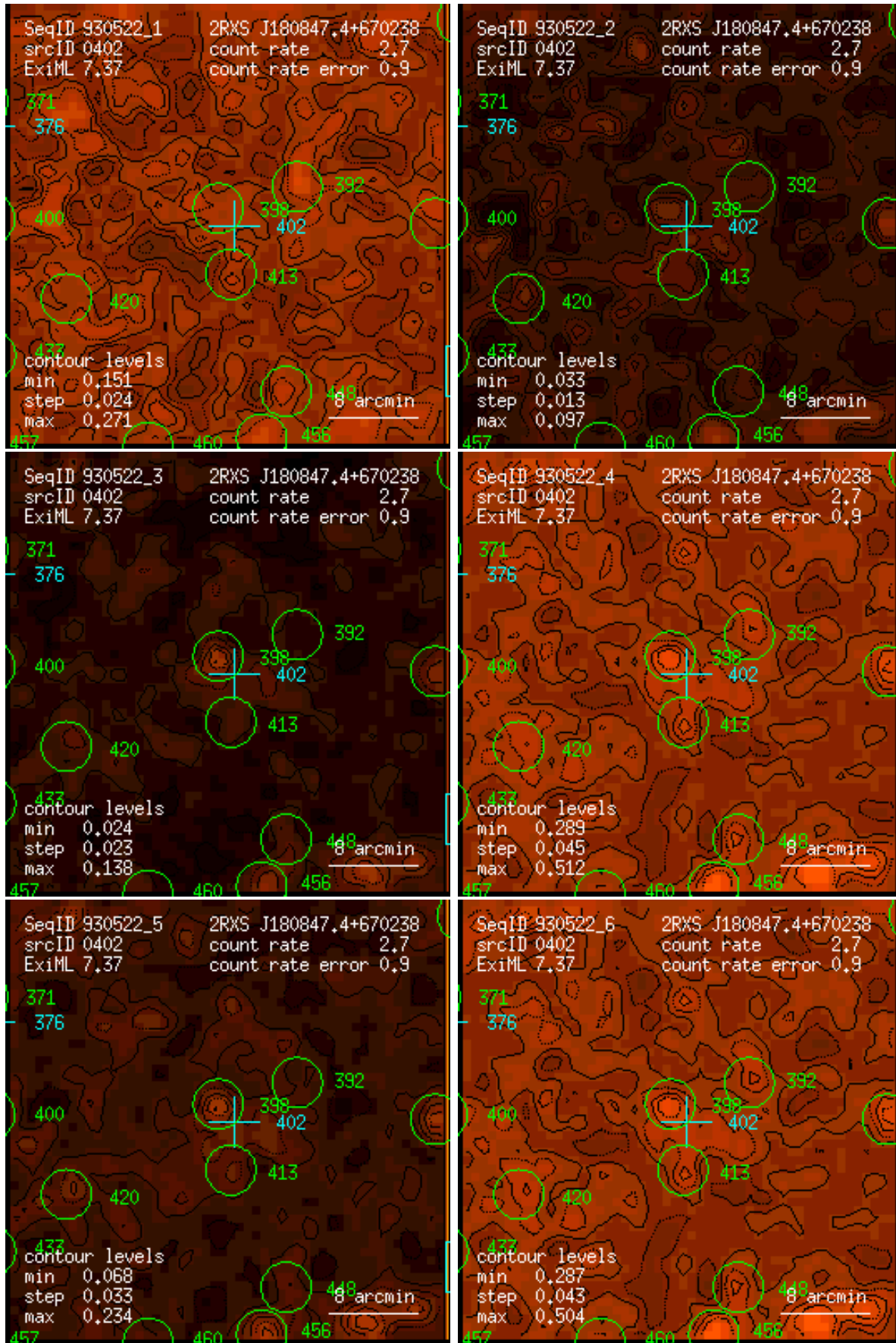
Figure 402: RASS 930522: detection 0402: band rate images, Gaussian filter: (1) PSPC channels 11 – 41, (2) 52 – 90, (3) 91 – 201, (4) 11 – 235, (5) 52 – 201, (6) 11 – 201. Broad band rates in counts/ks. Band rate contour levels in counts/ks/arcmin 2 .
