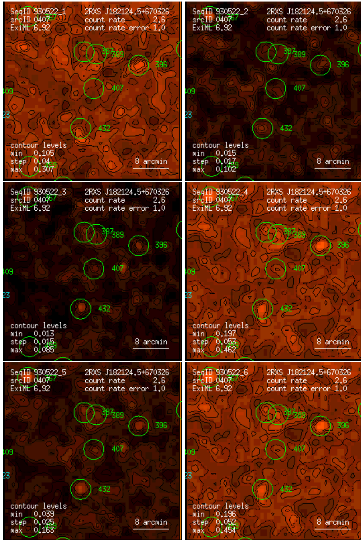
Figure 407: RASS 930522: detection 0407: band rate images, Gaussian filter: (1) PSPC channels 11 – 41, (2) 52 – 90, (3) 91 – 201, (4) 11 – 235, (5) 52 – 201, (6) 11 – 201. Broad band rates in counts/ks. Band rate contour levels in counts/ks/arcmin 2 .
