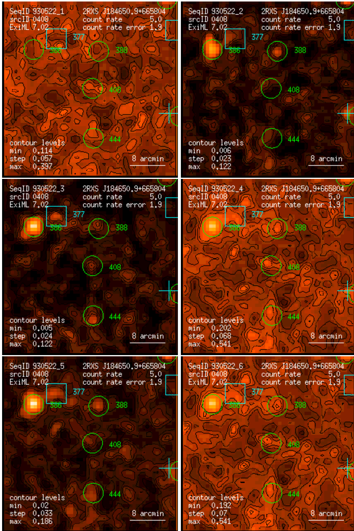
Figure 408: RASS 930522: detection 0408: band rate images, Gaussian filter: (1) PSPC channels 11 – 41, (2) 52 – 90, (3) 91 – 201, (4) 11 – 235, (5) 52 – 201, (6) 11 – 201. Broad band rates in counts/ks. Band rate contour levels in counts/ks/arcmin 2 .
