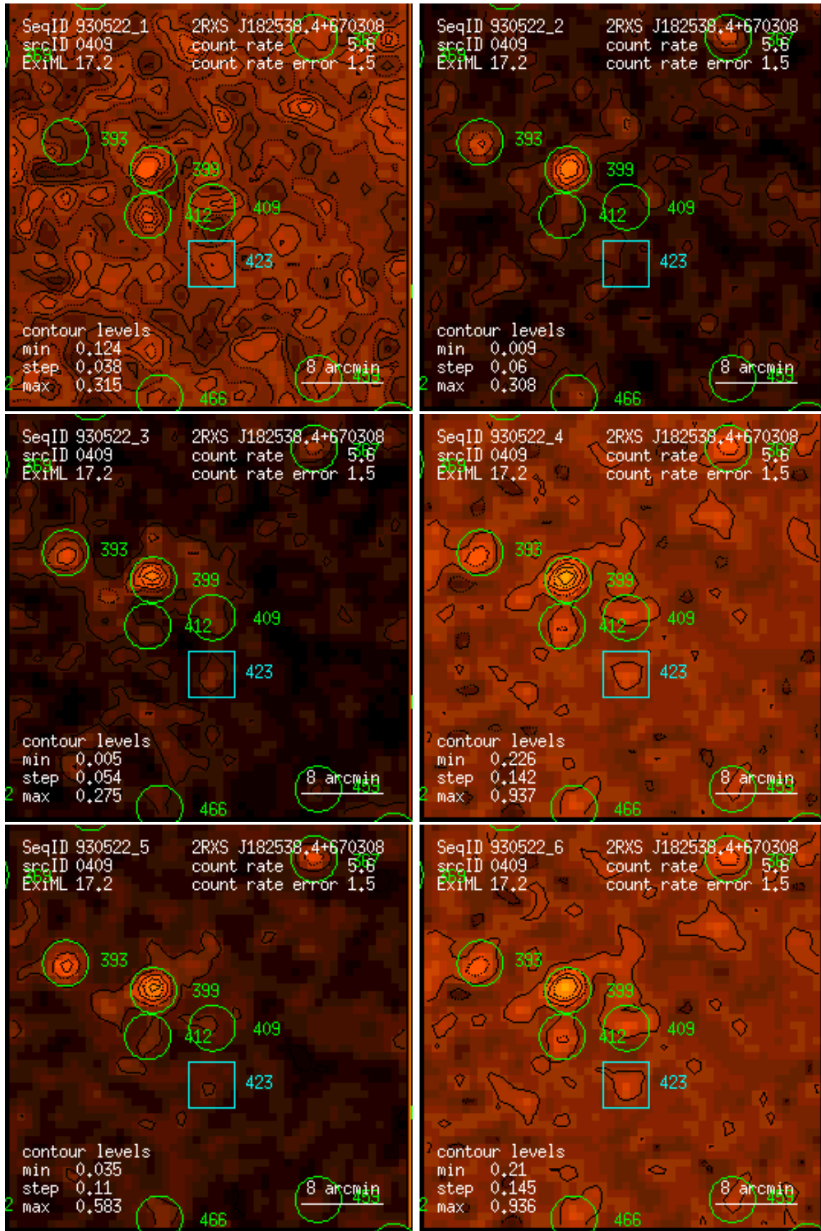
Figure 409: RASS 930522: detection 0409: band rate images, Gaussian filter: (1) PSPC channels 11 – 41, (2) 52 – 90, (3) 91 – 201, (4) 11 – 235, (5) 52 – 201, (6) 11 – 201. Broad band rates in counts/ks. Band rate contour levels in counts/ks/arcmin 2 .
