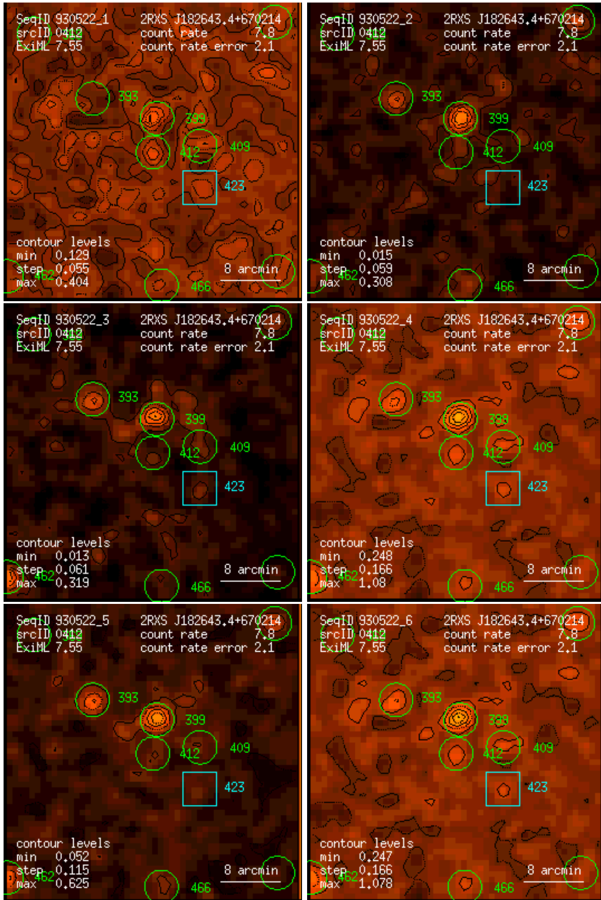
Figure 412: RASS 930522: detection 0412: band rate images, Gaussian filter: (1) PSPC channels 11 – 41, (2) 52 – 90, (3) 91 – 201, (4) 11 – 235, (5) 52 – 201, (6) 11 – 201. Broad band rates in counts/ks. Band rate contour levels in counts/ks/arcmin 2 .
