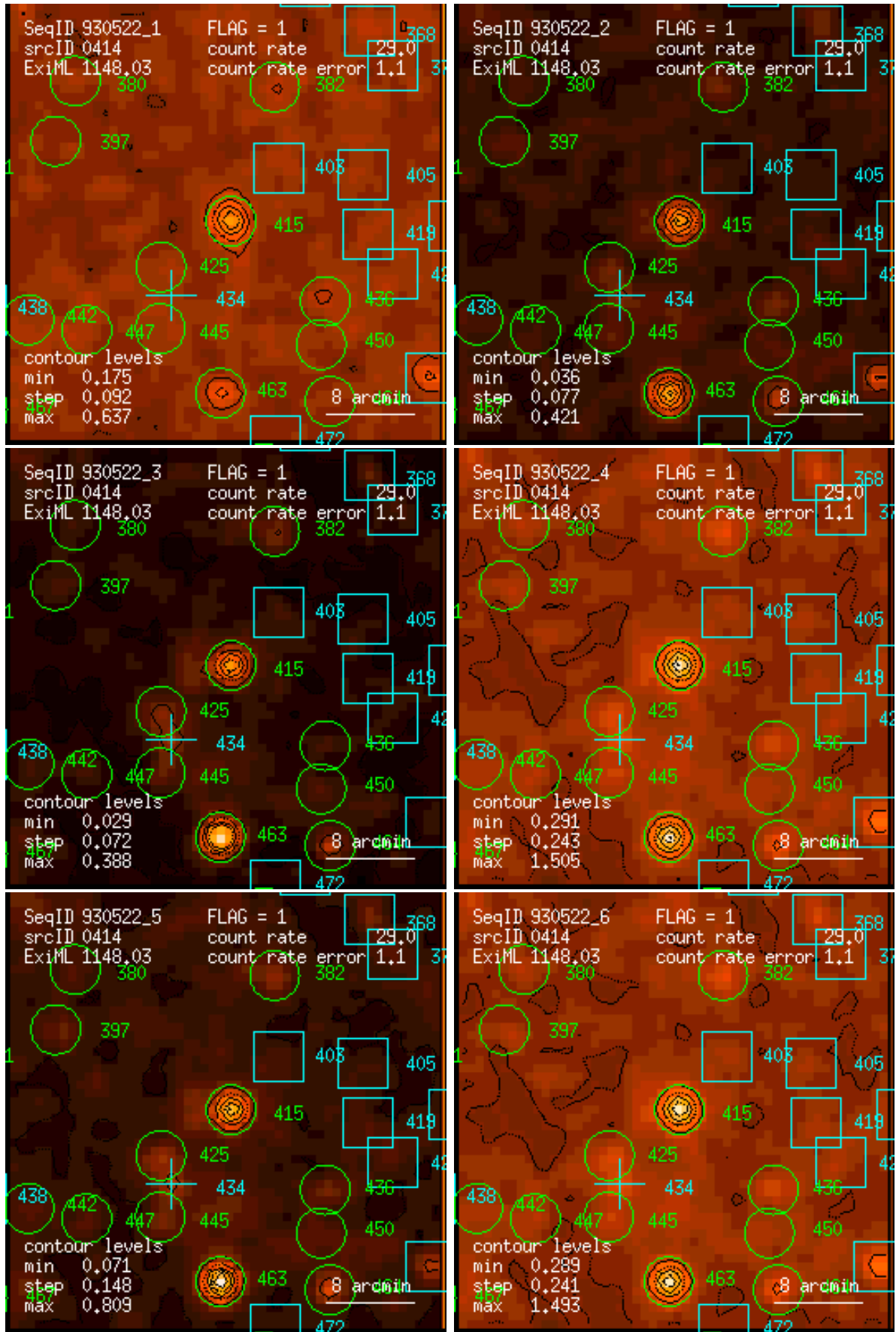
Figure 414: RASS 930522: detection 0414: band rate images, Gaussian filter: (1) PSPC channels 11 – 41, (2) 52 – 90, (3) 91 – 201, (4) 11 – 235, (5) 52 – 201, (6) 11 – 201. Broad band rates in counts/ks. Band rate contour levels in counts/ks/arcmin 2 .
