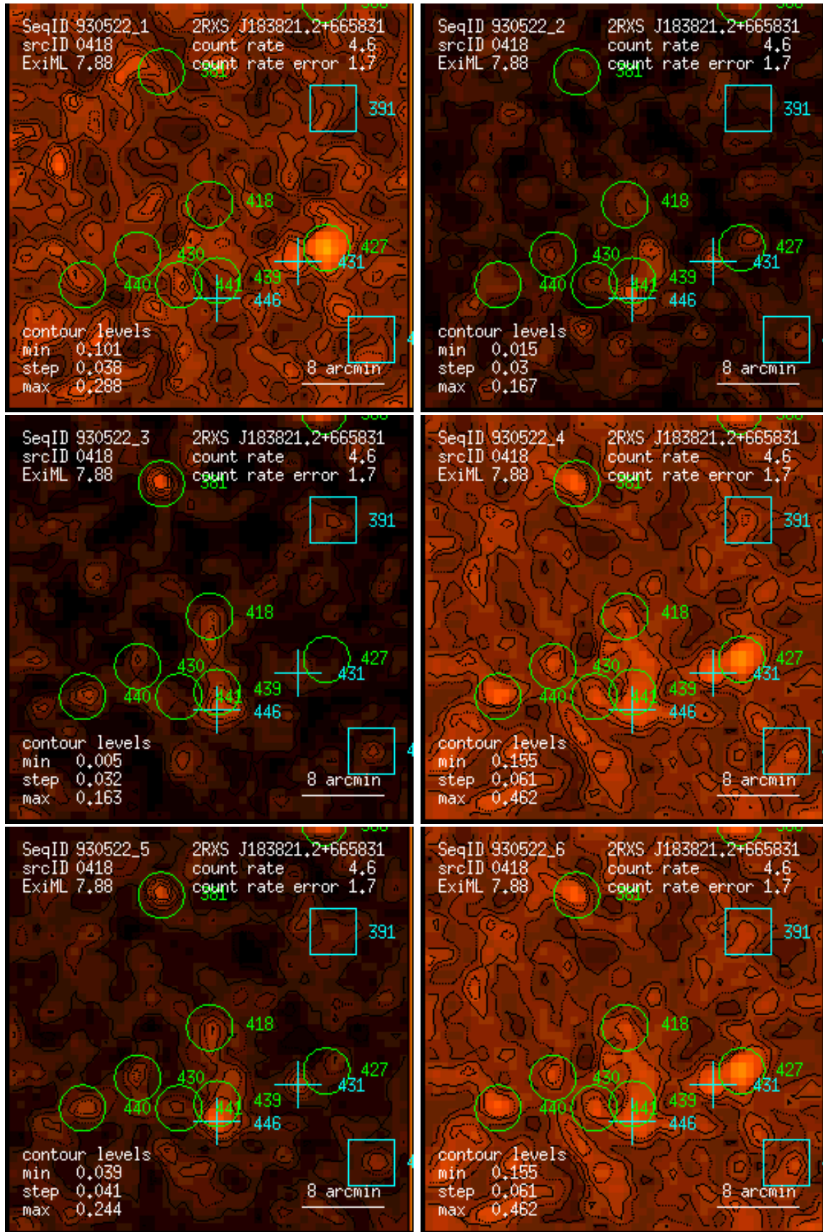
Figure 418: RASS 930522: detection 0418: band rate images, Gaussian filter: (1) PSPC channels 11 – 41, (2) 52 – 90, (3) 91 – 201, (4) 11 – 235, (5) 52 – 201, (6) 11 – 201. Broad band rates in counts/ks. Band rate contour levels in counts/ks/arcmin 2 .
