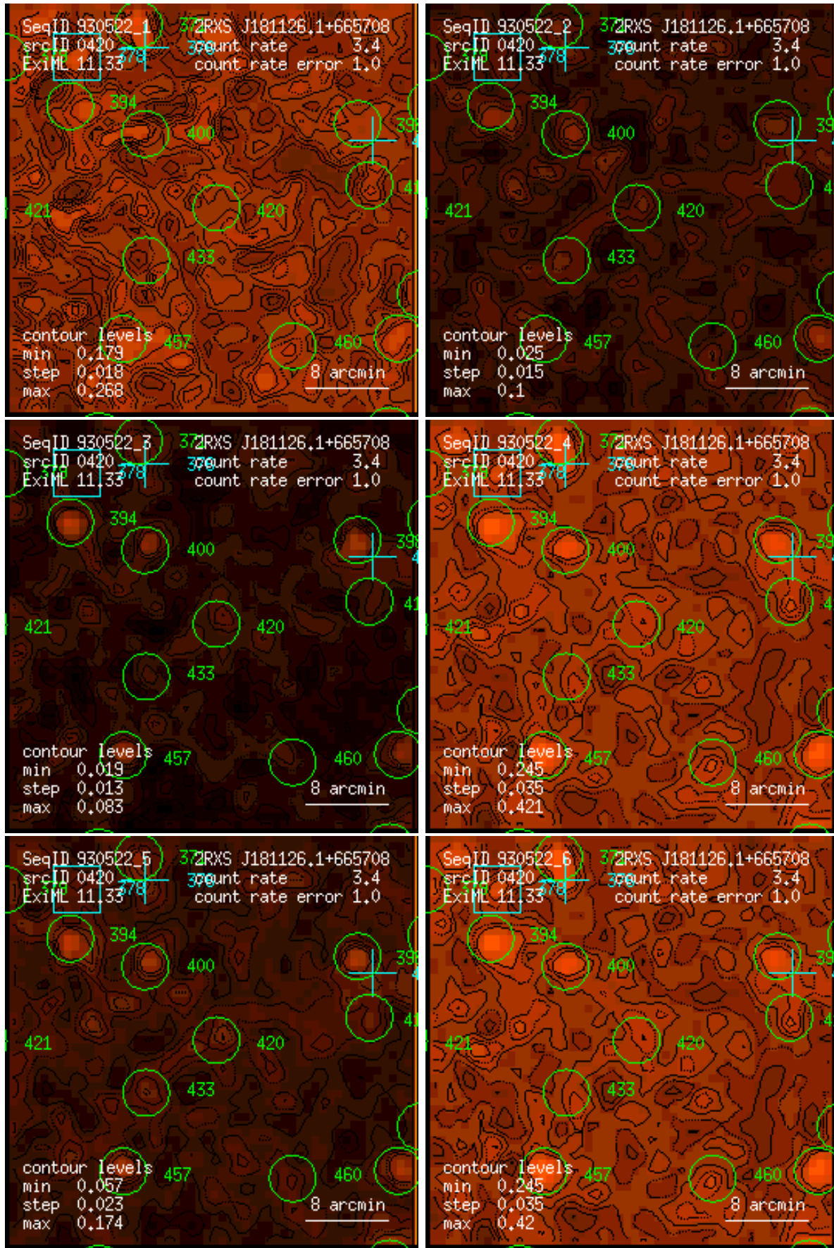
Figure 420: RASS 930522: detection 0420: band rate images, Gaussian filter: (1) PSPC channels 11 – 41, (2) 52 – 90, (3) 91 – 201, (4) 11 – 235, (5) 52 – 201, (6) 11 – 201. Broad band rates in counts/ks. Band rate contour levels in counts/ks/arcmin 2 .
