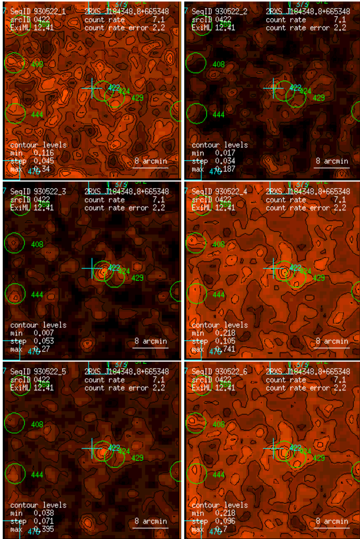
Figure 422: RASS 930522: detection 0422: band rate images, Gaussian filter: (1) PSPC channels 11 – 41, (2) 52 – 90, (3) 91 – 201, (4) 11 – 235, (5) 52 – 201, (6) 11 – 201. Broad band rates in counts/ks. Band rate contour levels in counts/ks/arcmin 2 .
