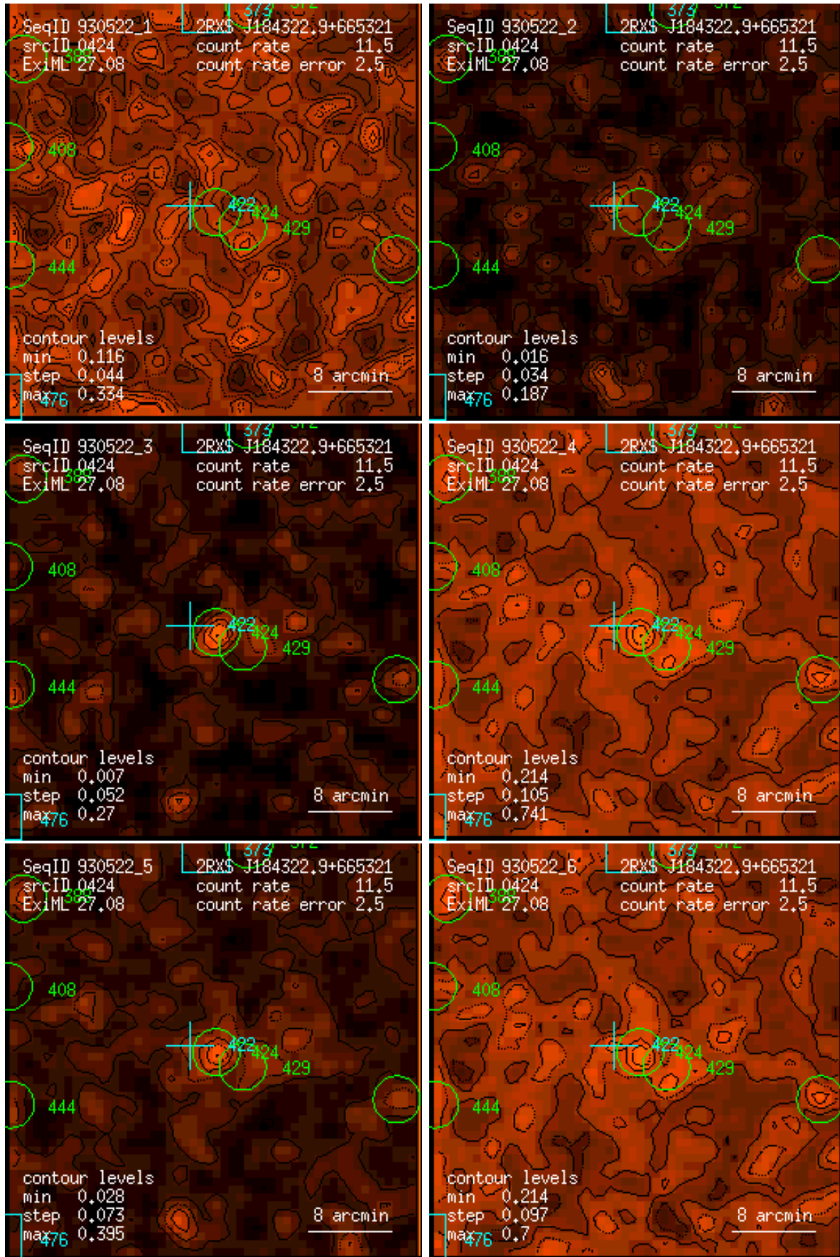
Figure 424: RASS 930522: detection 0424: band rate images, Gaussian filter: (1) PSPC channels 11 – 41, (2) 52 – 90, (3) 91 – 201, (4) 11 – 235, (5) 52 – 201, (6) 11 – 201. Broad band rates in counts/ks. Band rate contour levels in counts/ks/arcmin 2 .
