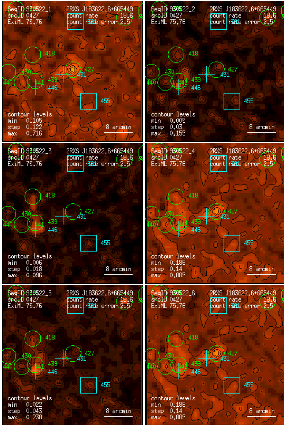
Figure 427: RASS 930522: detection 0427: band rate images, Gaussian filter: (1) PSPC channels 11 – 41, (2) 52 – 90, (3) 91 – 201, (4) 11 – 235, (5) 52 – 201, (6) 11 – 201. Broad band rates in counts/ks. Band rate contour levels in counts/ks/arcmin 2 .
