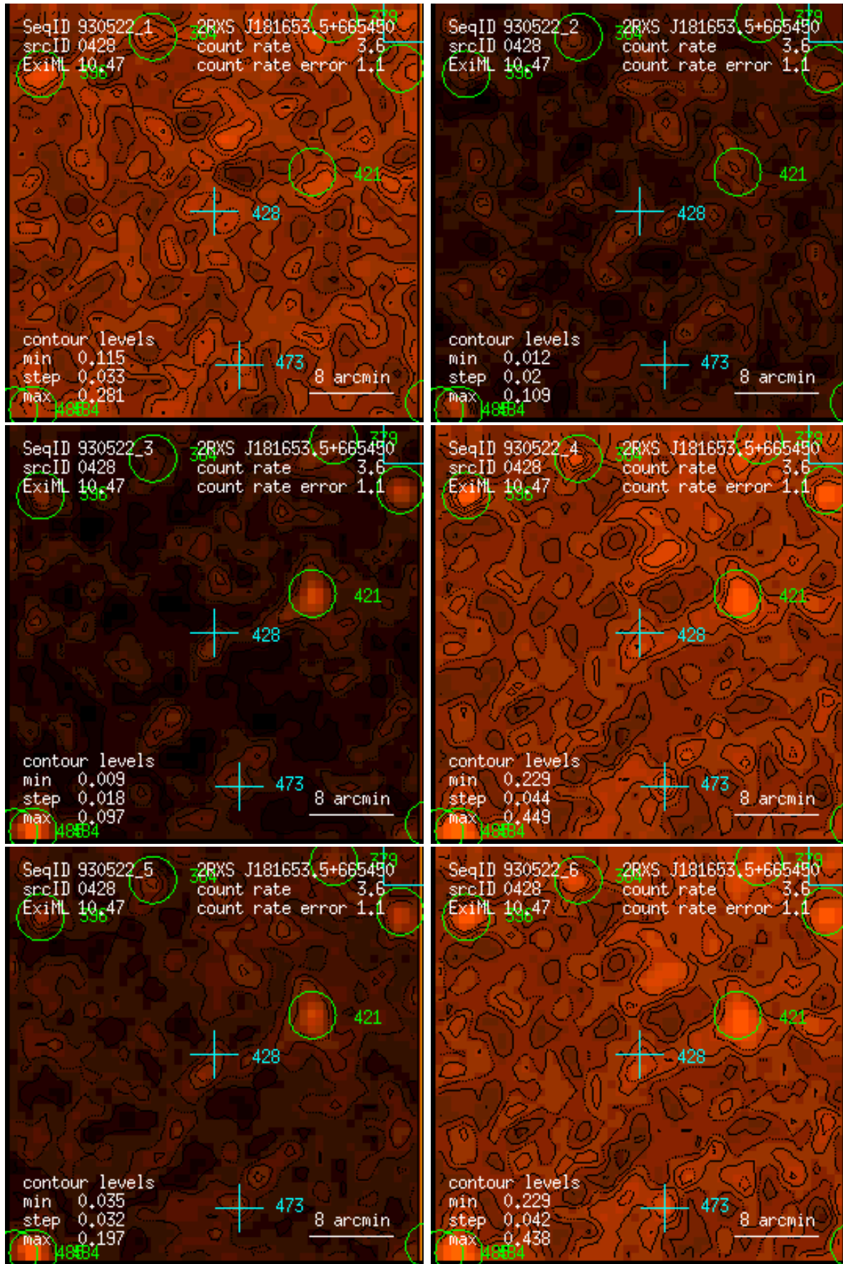
Figure 428: RASS 930522: detection 0428: band rate images, Gaussian filter: (1) PSPC channels 11 – 41, (2) 52 – 90, (3) 91 – 201, (4) 11 – 235, (5) 52 – 201, (6) 11 – 201. Broad band rates in counts/ks. Band rate contour levels in counts/ks/arcmin 2 .
