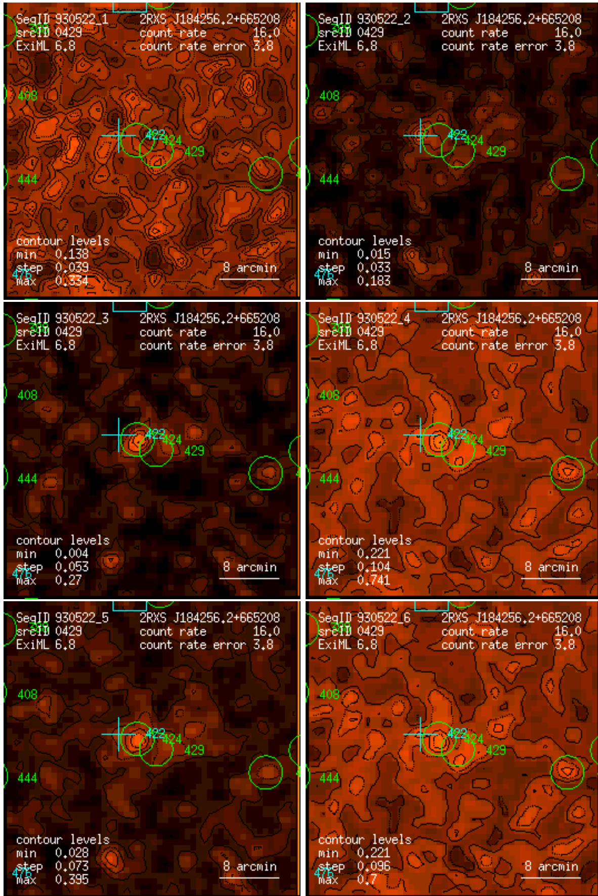
Figure 429: RASS 930522: detection 0429: band rate images, Gaussian filter: (1) PSPC channels 11 – 41, (2) 52 – 90, (3) 91 – 201, (4) 11 – 235, (5) 52 – 201, (6) 11 – 201. Broad band rates in counts/ks. Band rate contour levels in counts/ks/arcmin 2 .
