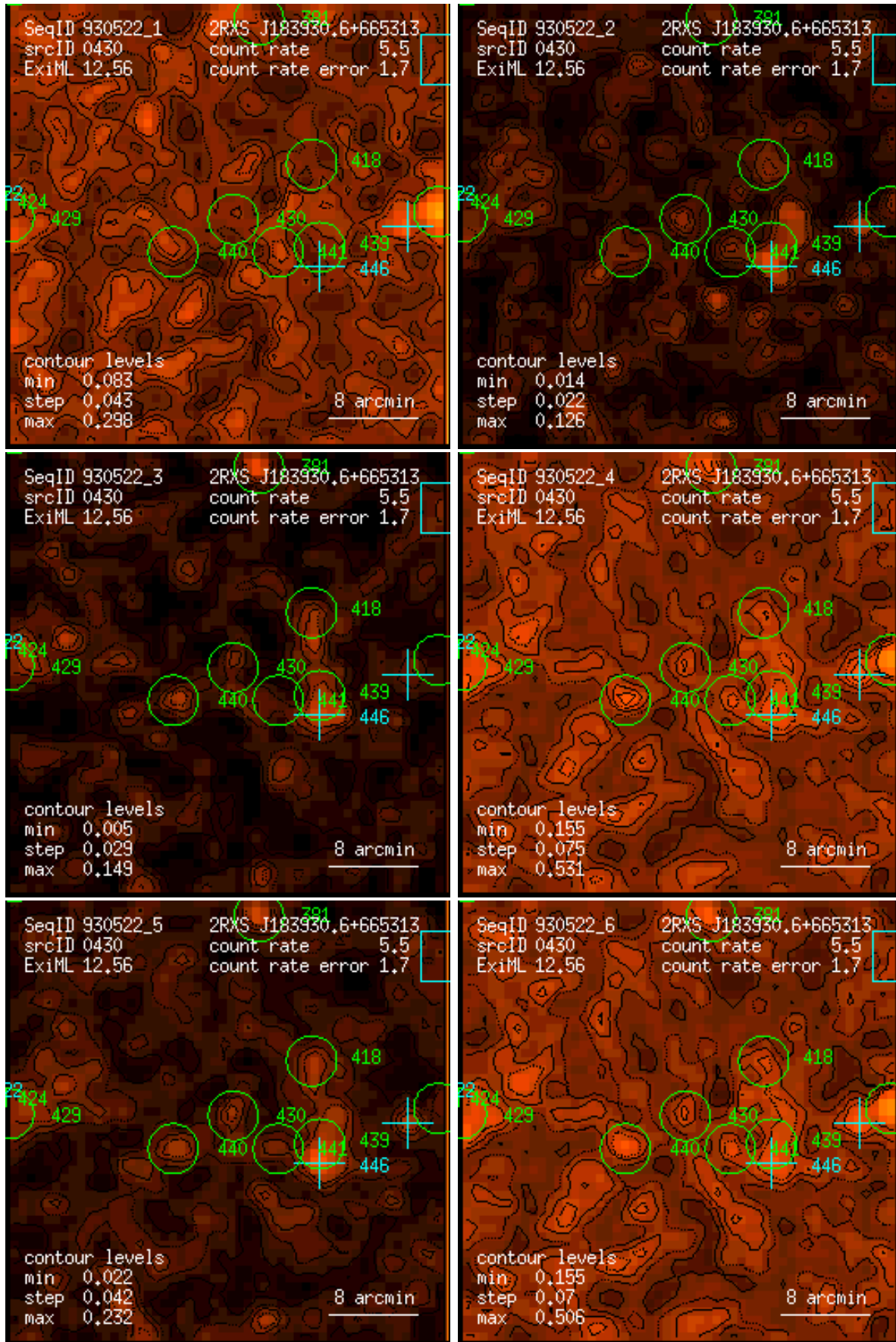
Figure 430: RASS 930522: detection 0430: band rate images, Gaussian filter: (1) PSPC channels 11 – 41, (2) 52 – 90, (3) 91 – 201, (4) 11 – 235, (5) 52 – 201, (6) 11 – 201. Broad band rates in counts/ks. Band rate contour levels in counts/ks/arcmin 2 .
