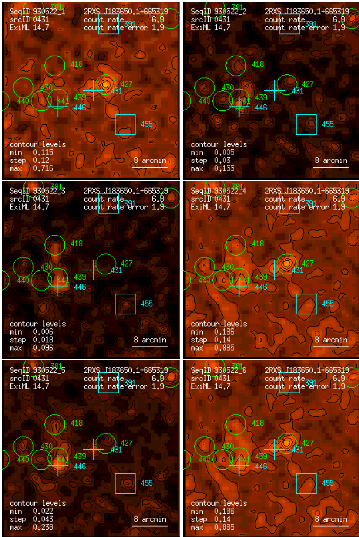
Figure 431: RASS 930522: detection 0431: band rate images, Gaussian filter: (1) PSPC channels 11 – 41, (2) 52 – 90, (3) 91 – 201, (4) 11 – 235, (5) 52 – 201, (6) 11 – 201. Broad band rates in counts/ks. Band rate contour levels in counts/ks/arcmin 2 .
