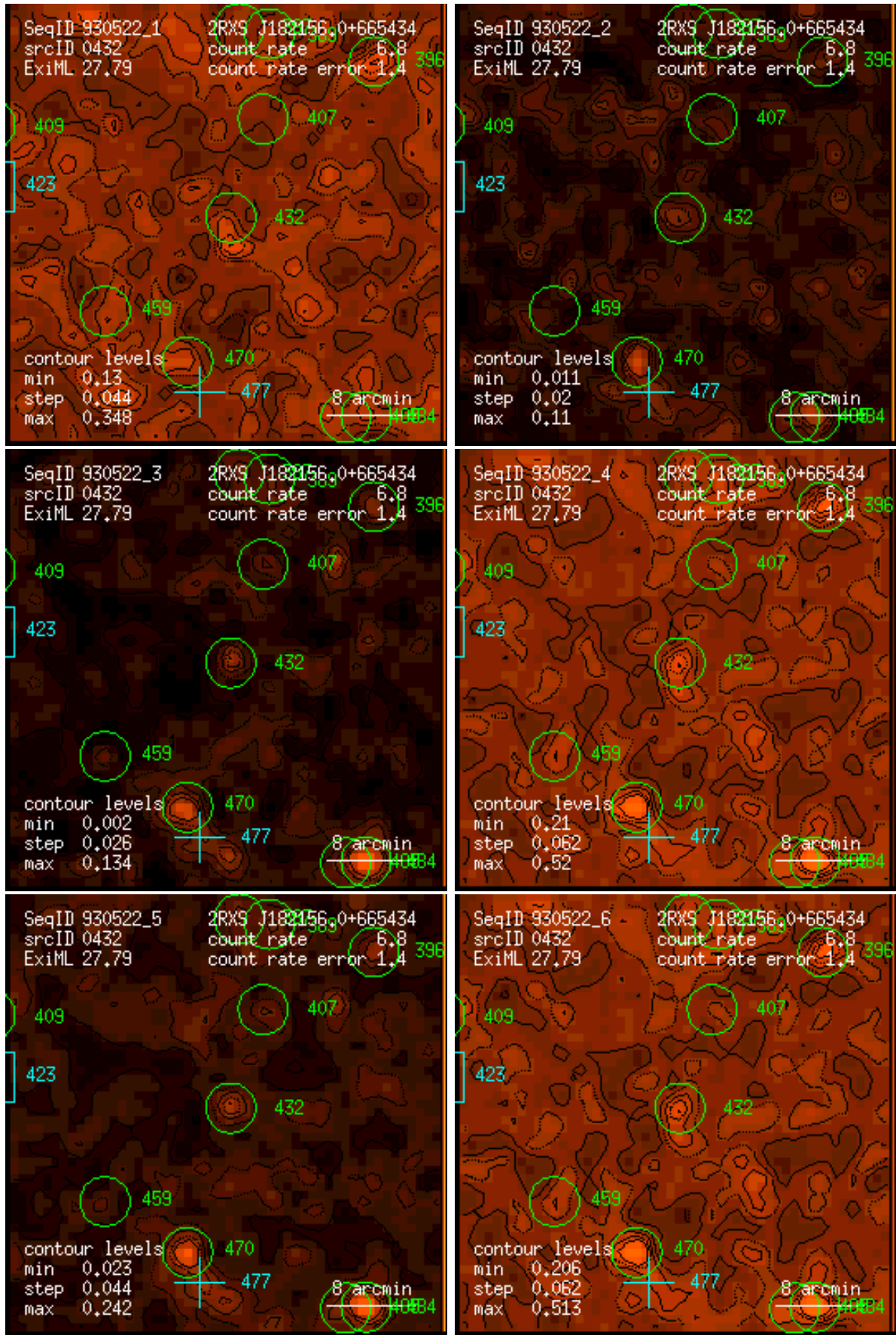
Figure 432: RASS 930522: detection 0432: band rate images, Gaussian filter: (1) PSPC channels 11 – 41, (2) 52 – 90, (3) 91 – 201, (4) 11 – 235, (5) 52 – 201, (6) 11 – 201. Broad band rates in counts/ks. Band rate contour levels in counts/ks/arcmin 2 .
