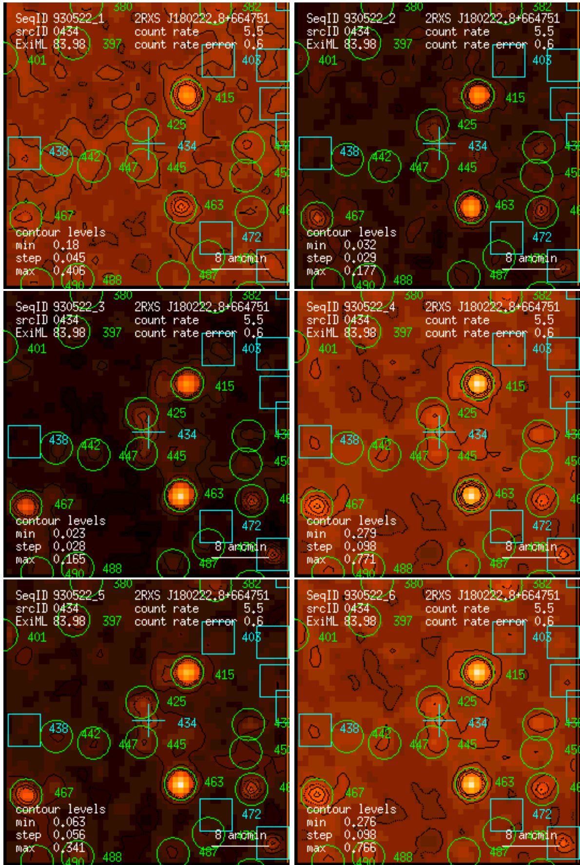
Figure 434: RASS 930522: detection 0434: band rate images, Gaussian filter: (1) PSPC channels 11 – 41, (2) 52 – 90, (3) 91 – 201, (4) 11 – 235, (5) 52 – 201, (6) 11 – 201. Broad band rates in counts/ks. Band rate contour levels in counts/ks/arcmin 2 .
