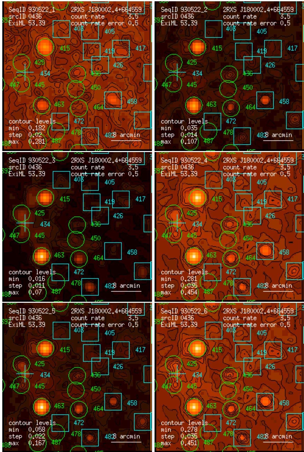
Figure 436: RASS 930522: detection 0436: band rate images, Gaussian filter: (1) PSPC channels 11 – 41, (2) 52 – 90, (3) 91 – 201, (4) 11 – 235, (5) 52 – 201, (6) 11 – 201. Broad band rates in counts/ks. Band rate contour levels in counts/ks/arcmin 2 .
