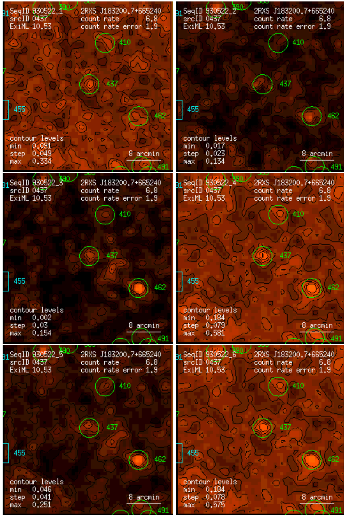
Figure 437: RASS 930522: detection 0437: band rate images, Gaussian filter: (1) PSPC channels 11 – 41, (2) 52 – 90, (3) 91 – 201, (4) 11 – 235, (5) 52 – 201, (6) 11 – 201. Broad band rates in counts/ks. Band rate contour levels in counts/ks/arcmin 2 .
