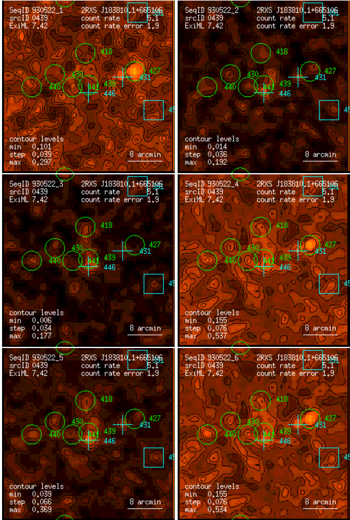
Figure 439: RASS 930522: detection 0439: band rate images, Gaussian filter: (1) PSPC channels 11 – 41, (2) 52 – 90, (3) 91 – 201, (4) 11 – 235, (5) 52 – 201, (6) 11 – 201. Broad band rates in counts/ks. Band rate contour levels in counts/ks/arcmin 2 .
