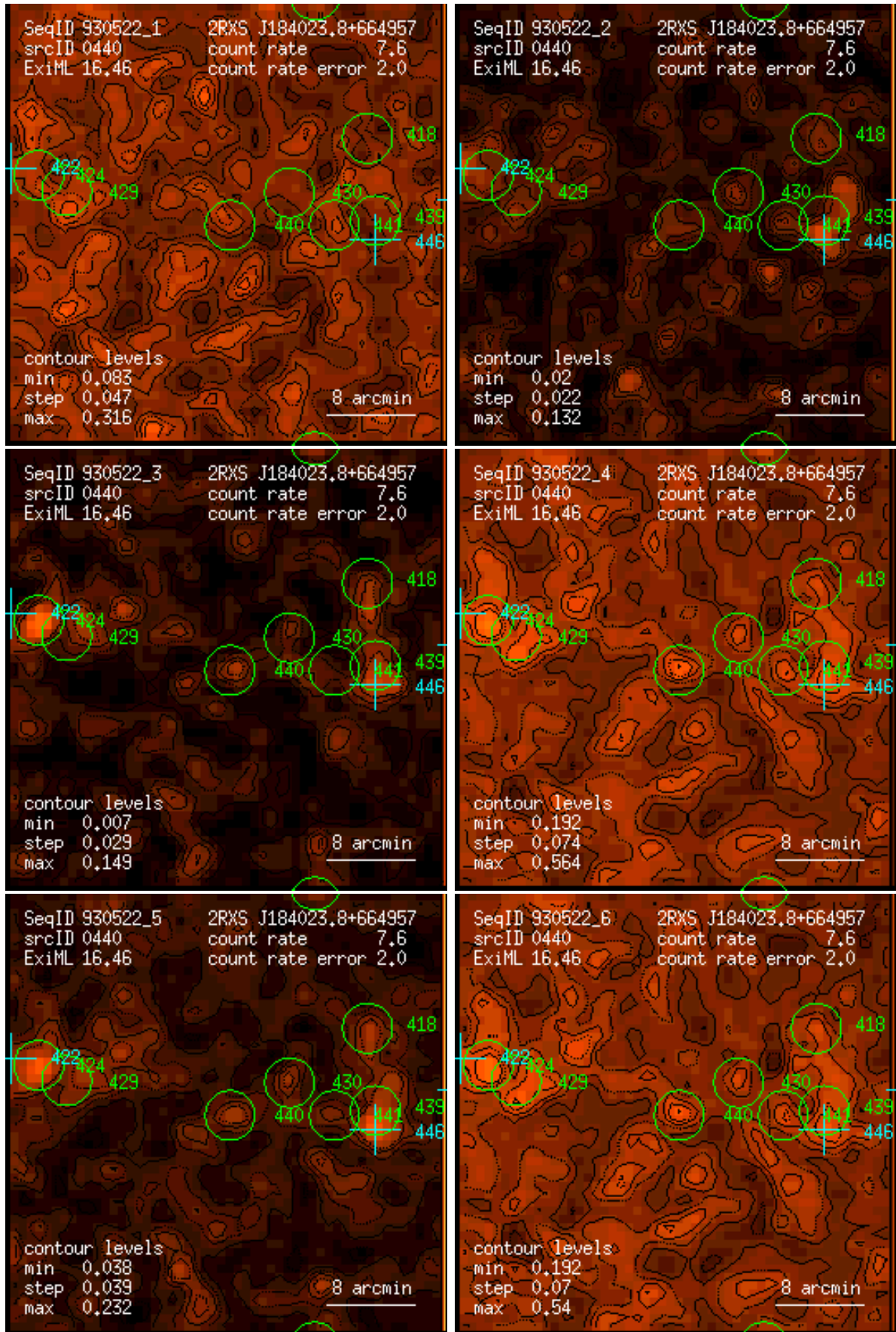
Figure 440: RASS 930522: detection 0440: band rate images, Gaussian filter: (1) PSPC channels 11 – 41, (2) 52 – 90, (3) 91 – 201, (4) 11 – 235, (5) 52 – 201, (6) 11 – 201. Broad band rates in counts/ks. Band rate contour levels in counts/ks/arcmin 2 .
