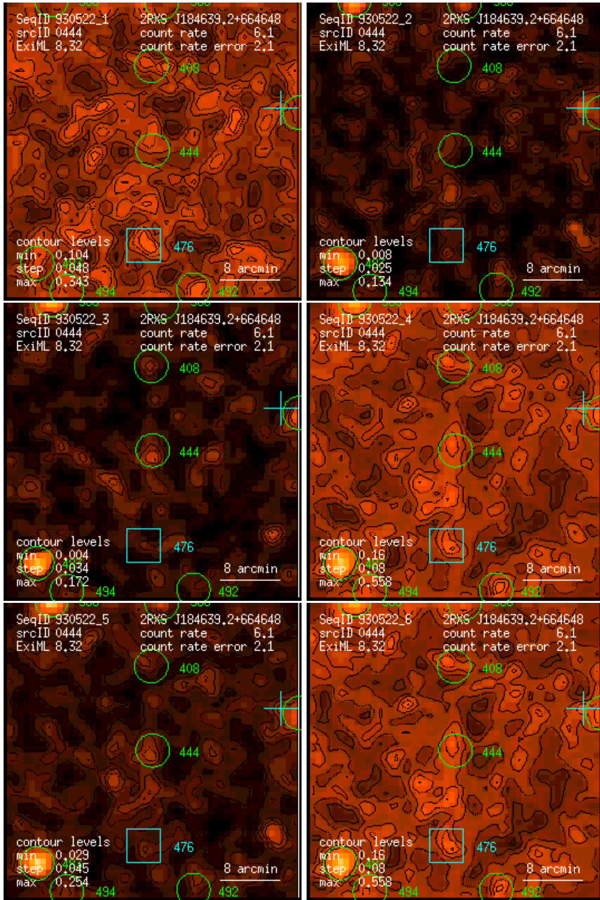
Figure 444: RASS 930522: detection 0444: band rate images, Gaussian filter: (1) PSPC channels 11 – 41, (2) 52 – 90, (3) 91 – 201, (4) 11 – 235, (5) 52 – 201, (6) 11 – 201. Broad band rates in counts/ks. Band rate contour levels in counts/ks/arcmin 2 .
