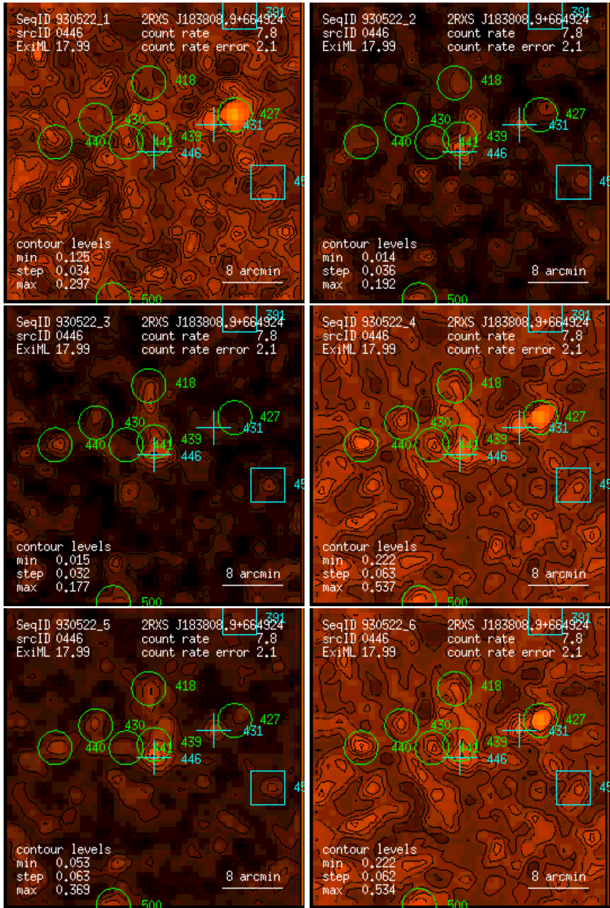
Figure 446: RASS 930522: detection 0446: band rate images, Gaussian filter: (1) PSPC channels 11 – 41, (2) 52 – 90, (3) 91 – 201, (4) 11 – 235, (5) 52 – 201, (6) 11 – 201. Broad band rates in counts/ks. Band rate contour levels in counts/ks/arcmin 2 .
