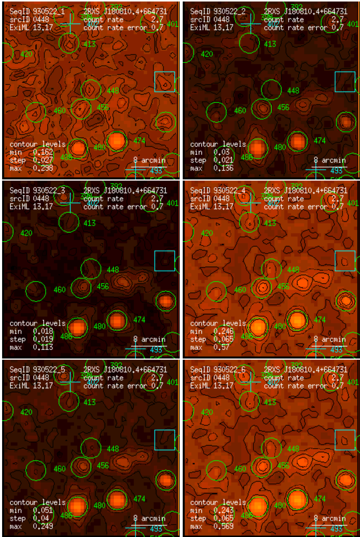
Figure 448: RASS 930522: detection 0448: band rate images, Gaussian filter: (1) PSPC channels 11 – 41, (2) 52 – 90, (3) 91 – 201, (4) 11 – 235, (5) 52 – 201, (6) 11 – 201. Broad band rates in counts/ks. Band rate contour levels in counts/ks/arcmin 2 .
