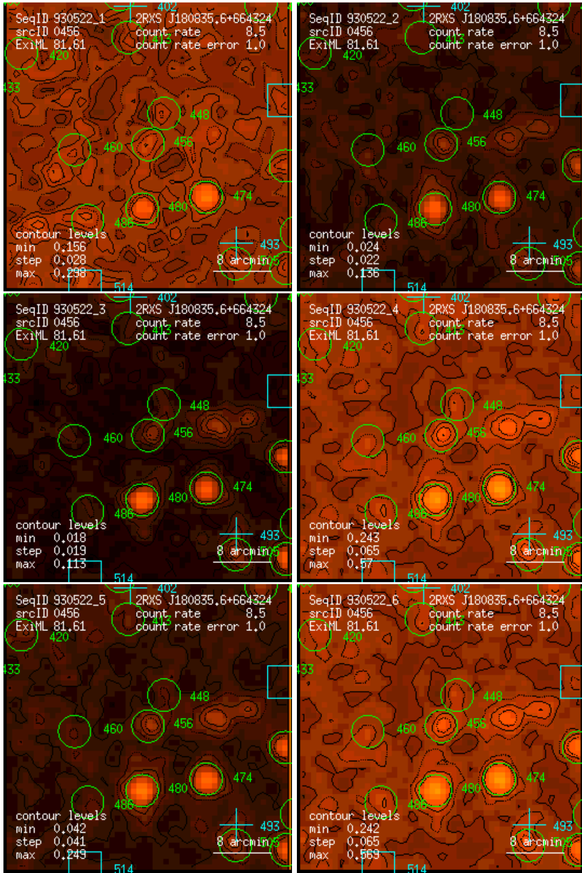
Figure 456: RASS 930522: detection 0456: band rate images, Gaussian filter: (1) PSPC channels 11 – 41, (2) 52 – 90, (3) 91 – 201, (4) 11 – 235, (5) 52 – 201, (6) 11 – 201. Broad band rates in counts/ks. Band rate contour levels in counts/ks/arcmin 2 .
