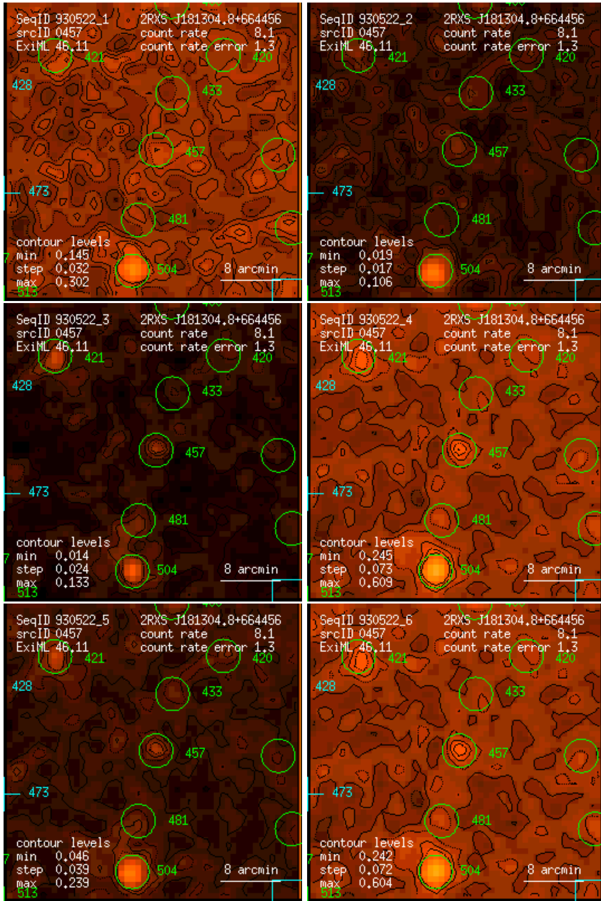
Figure 457: RASS 930522: detection 0457: band rate images, Gaussian filter: (1) PSPC channels 11 – 41, (2) 52 – 90, (3) 91 – 201, (4) 11 – 235, (5) 52 – 201, (6) 11 – 201. Broad band rates in counts/ks. Band rate contour levels in counts/ks/arcmin 2 .
